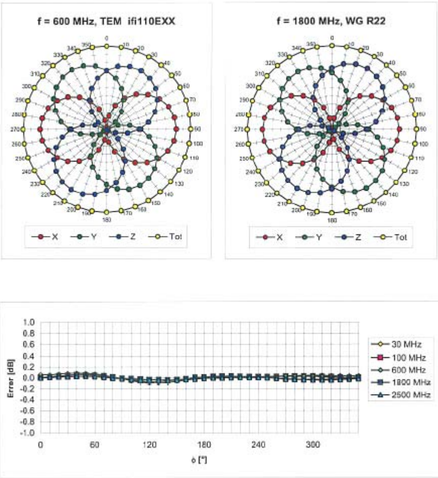
Uncertainty of Axial Isotropy Assessment: \pm 0.5\% ( k=2 )
