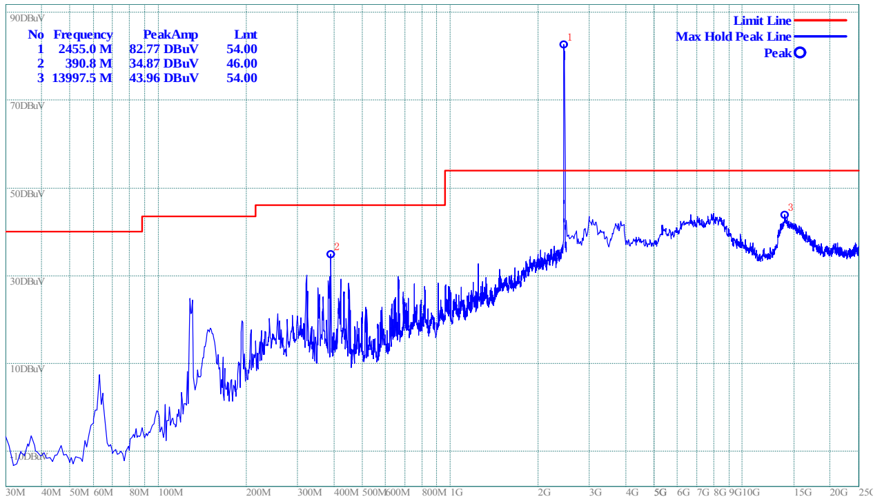
(Plot C.2: Antenna Horizontal, 30MHz to 25GHz)
