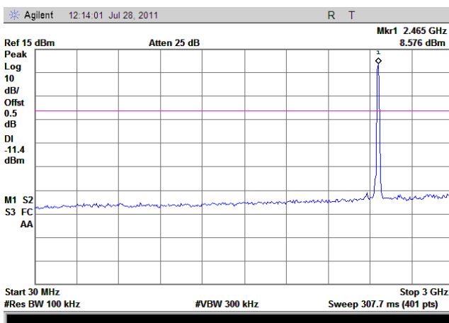
(Plot C.1: Channel = 11, 30MHz to 3GHz)
