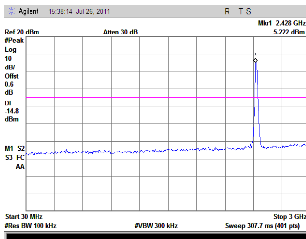
(Plot B.1: Channel = 6, 30MHz to 3GHz)
