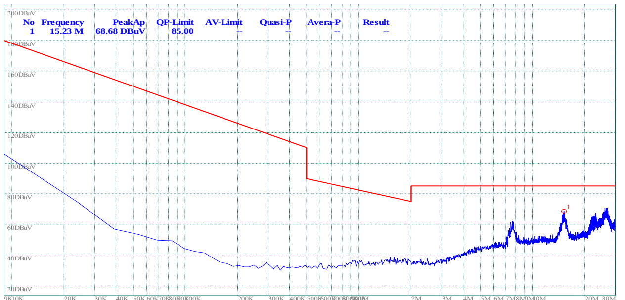
(Plot A.1: 9kHz to 30MHz)
