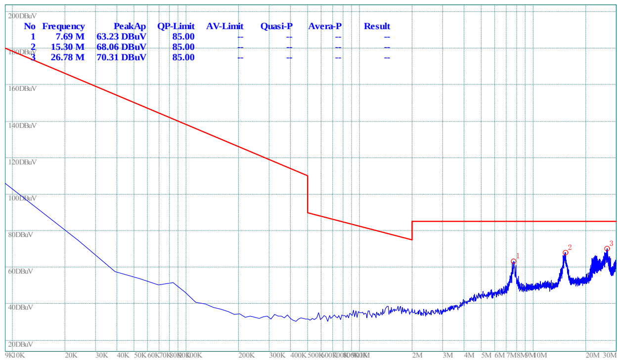
(Plot B.1: 9kHz to 30MHz)
