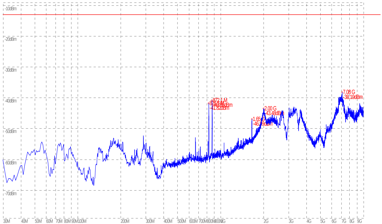
(Plot G.4: HSDPA 850MHz Channel = 4400, Test Antenna Vertical)
