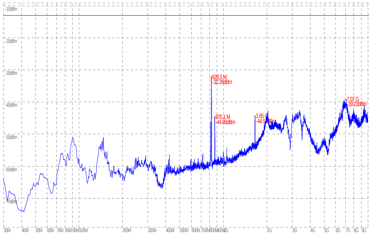
(Plot G.2: HSDPA 850MHz Channel = 4357, Test Antenna Vertical)
