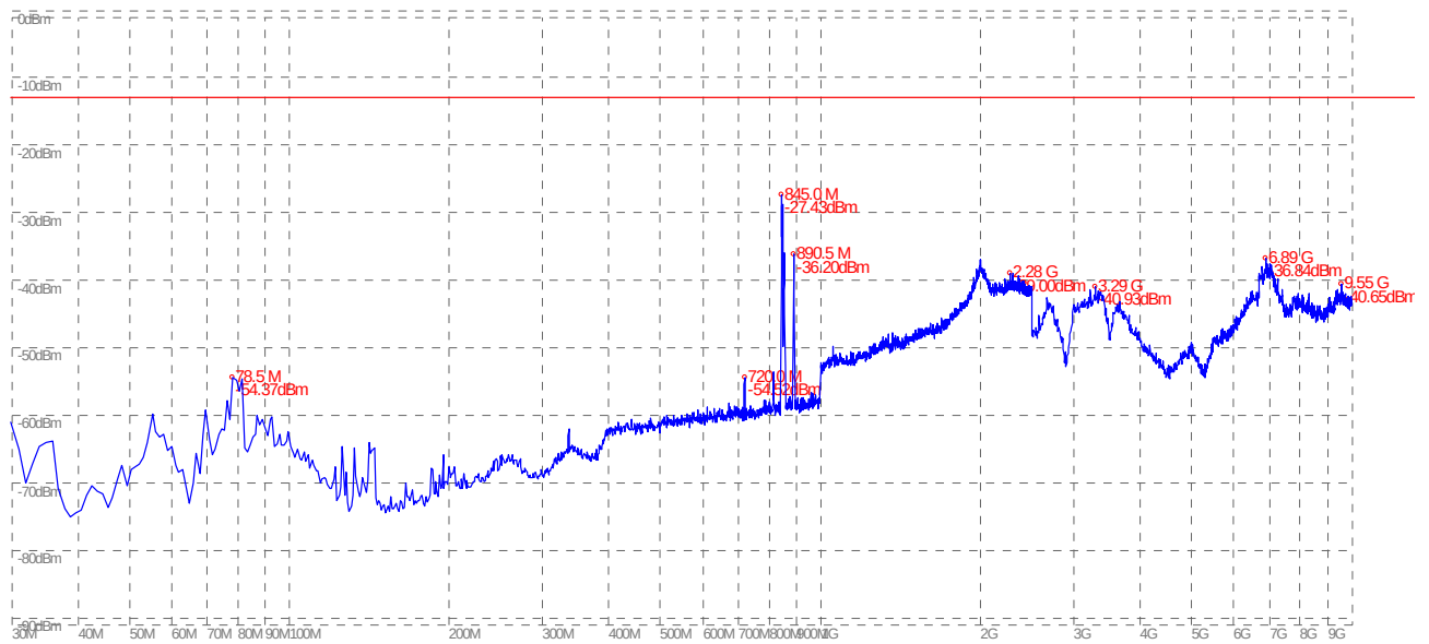
(Plot E.6: WCDMA 850MHz Channel = 4458, Test Antenna Vertical)
