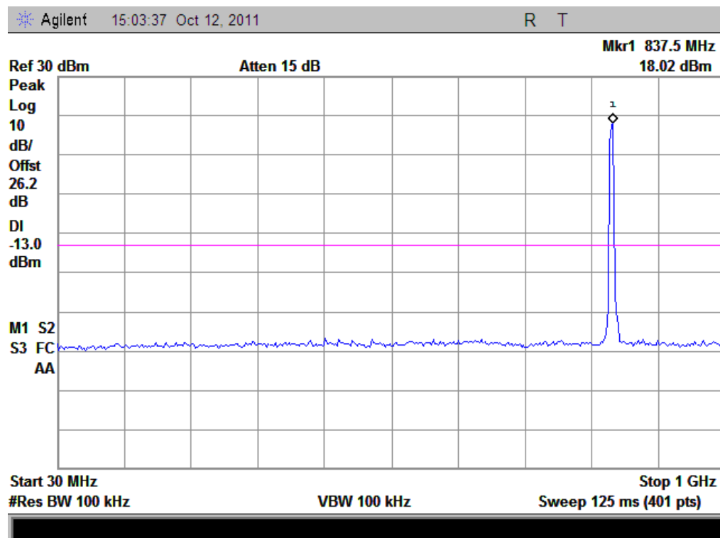
(Plot E2: WCDMA850MHz Channel = 4400, 30MHz to 1GHz)
