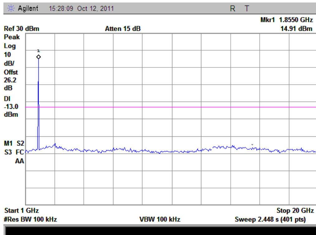
(Plot H1.1: HSDPA1900MHz Channel = 9662, 1GHz to 20GHz)
