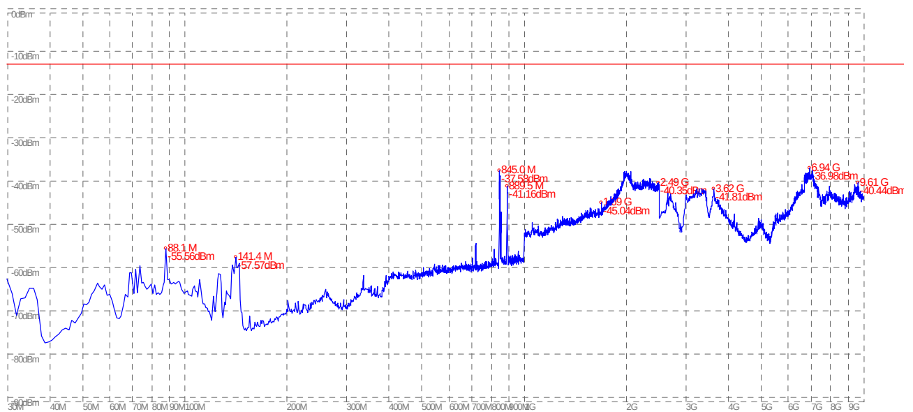
(Plot E.5: WCDMA 850MHz Channel = 4458, Test Antenna Horizontal)
