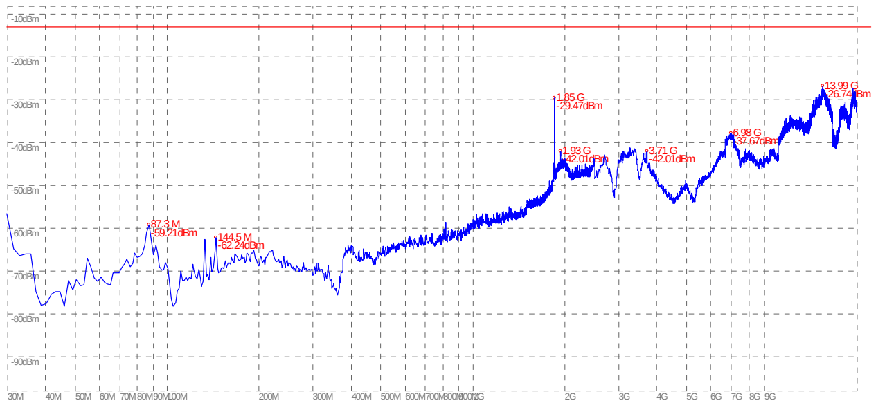
(Plot F.2: WCDMA 1900MHz Channel = 9662, Test Antenna Vertical)
