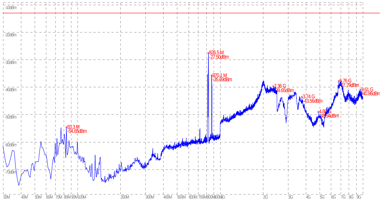
(Plot E.2: WCDMA 850MHz Channel = 4357, Test Antenna Vertical)
