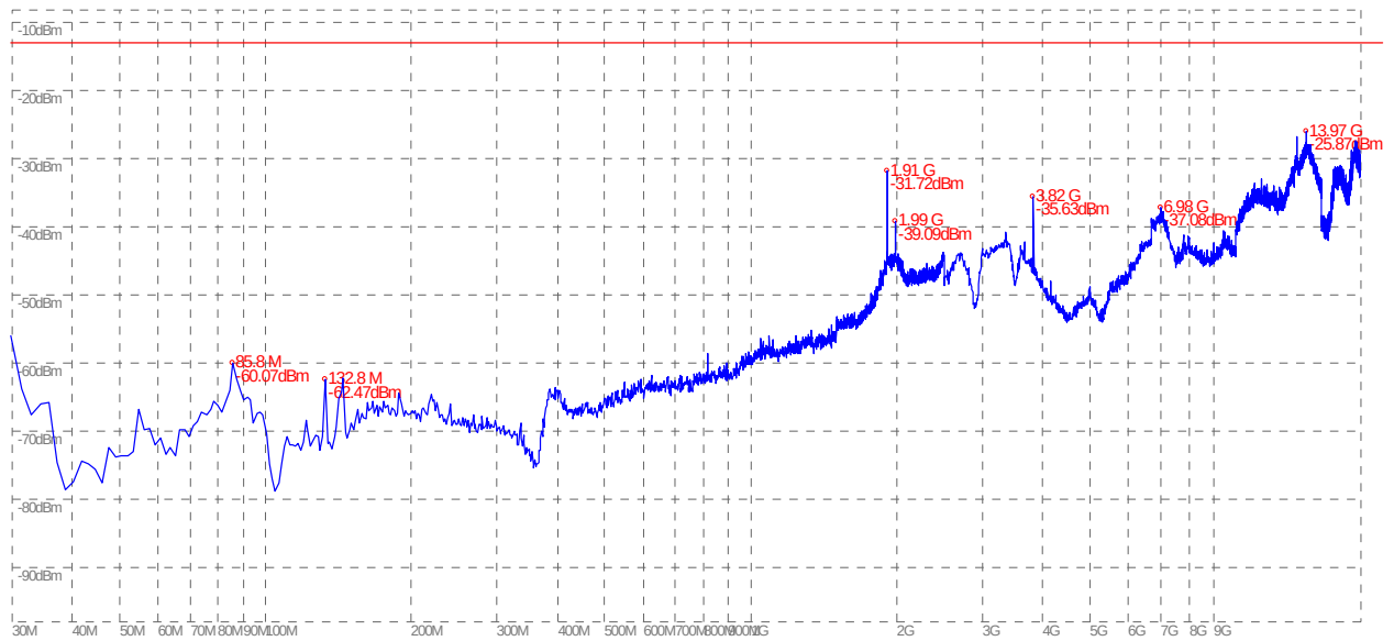
(Plot F.6: WCDMA 1900MHz Channel = 9938, Test Antenna Vertical)
