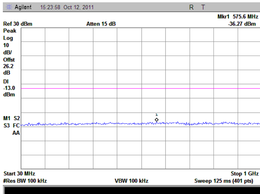
(Plot H3: HSDPA1900MHz Channel = 9938, 30MHz to 1GHz)
