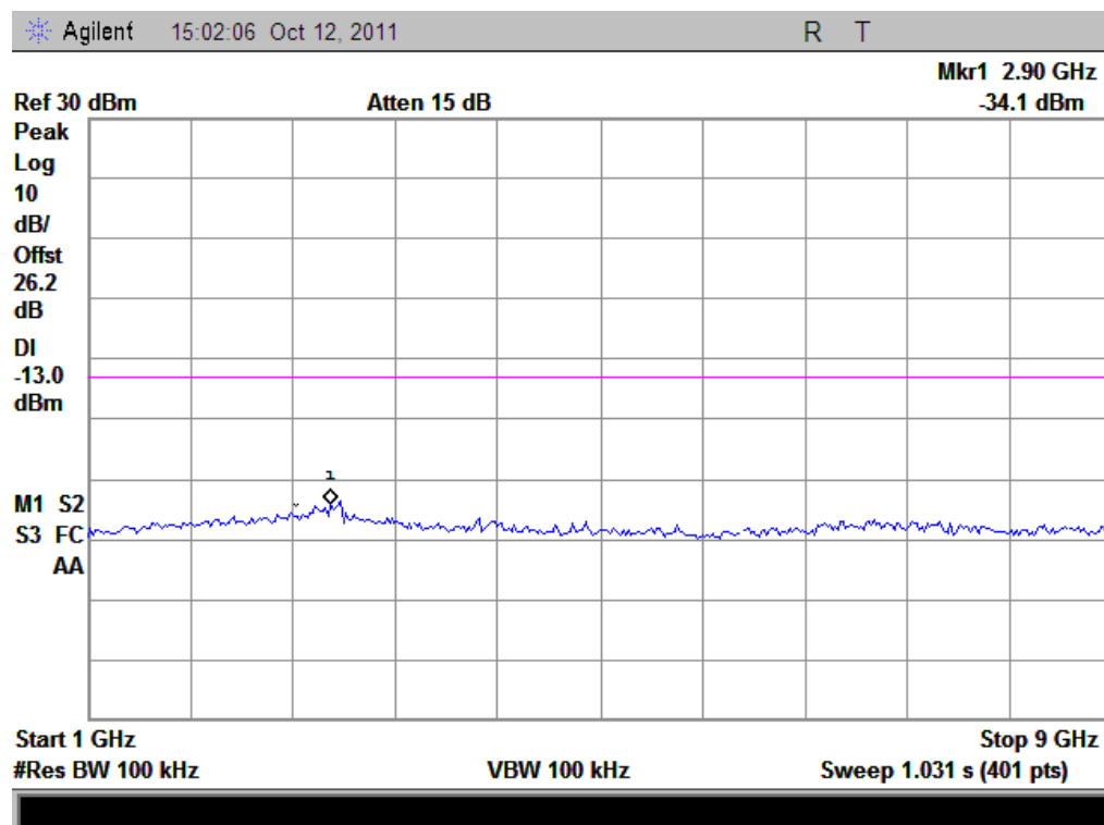
(Plot E1.1: WCDMA850MHz Channel = 4357, 1GHz to 9GHz)
