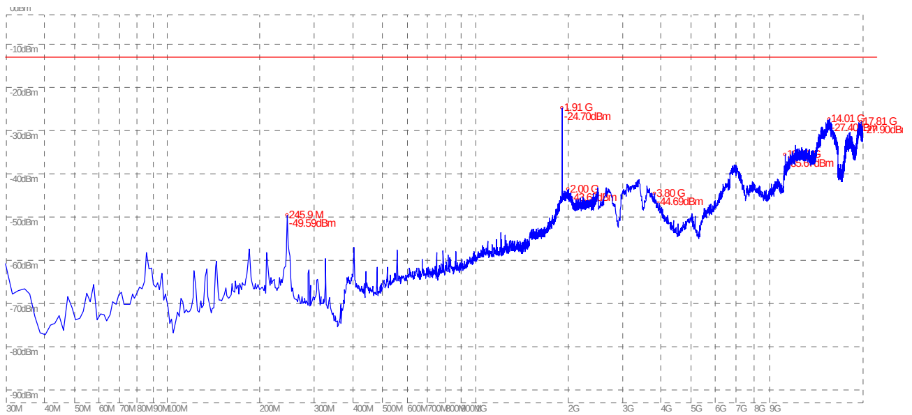
(PlotB.6: GSM 1900MHz Channel = 810, Test Antenna Vertical)
