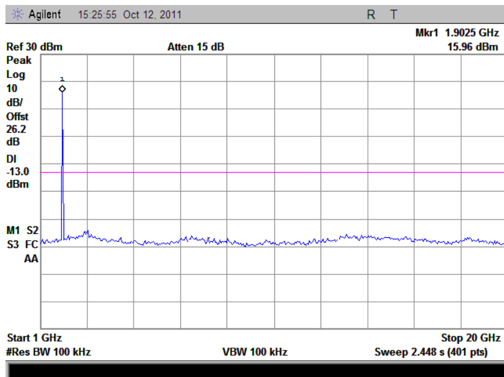
(Plot H3.1: HSDPA1900MHz Channel = 9938 1GHz to 20GHz)
