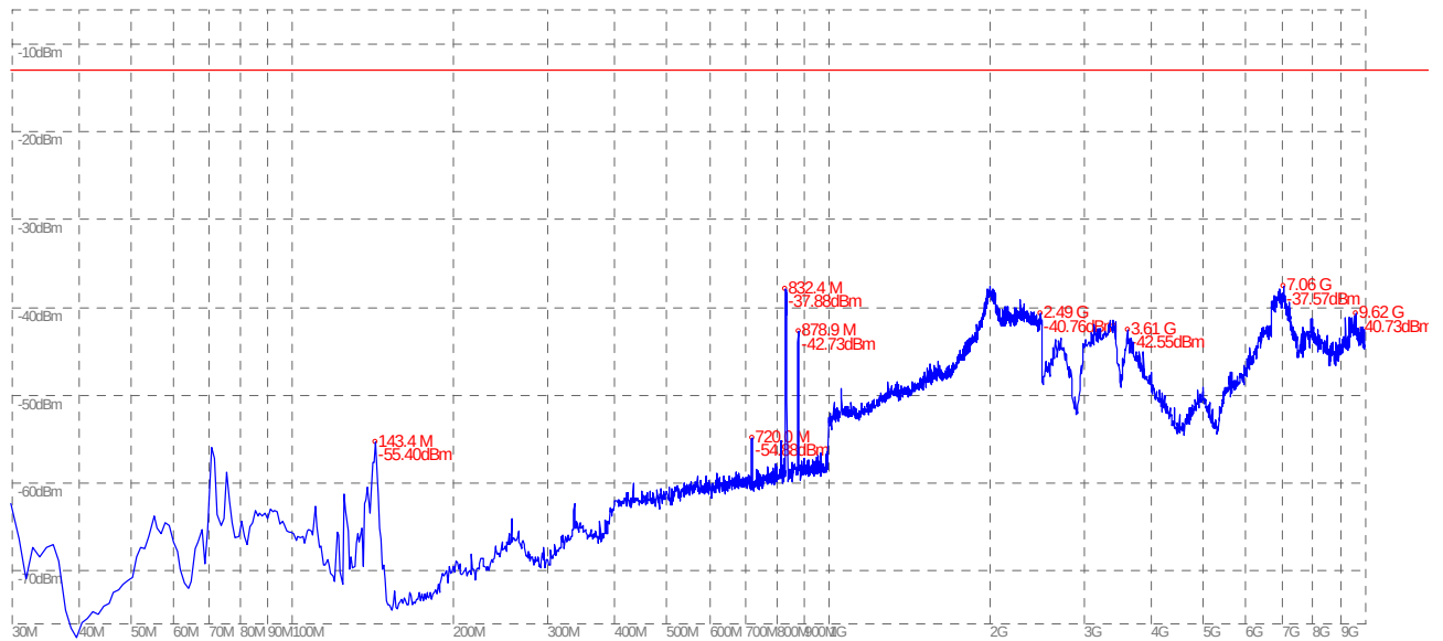
(Plot E.3: WCDMA 850MHz Channel = 4400, Test Antenna Horizontal)
