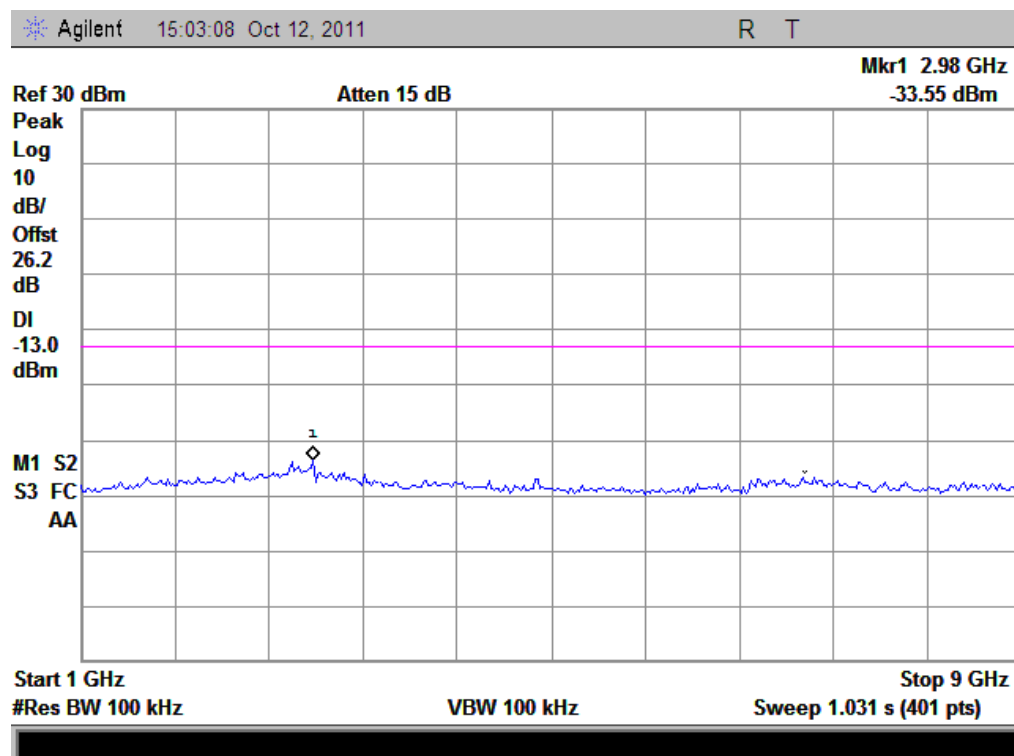
(Plot E2.1: WCDMA850MHz Channel = 4400, 1GHz to 9GHz)
