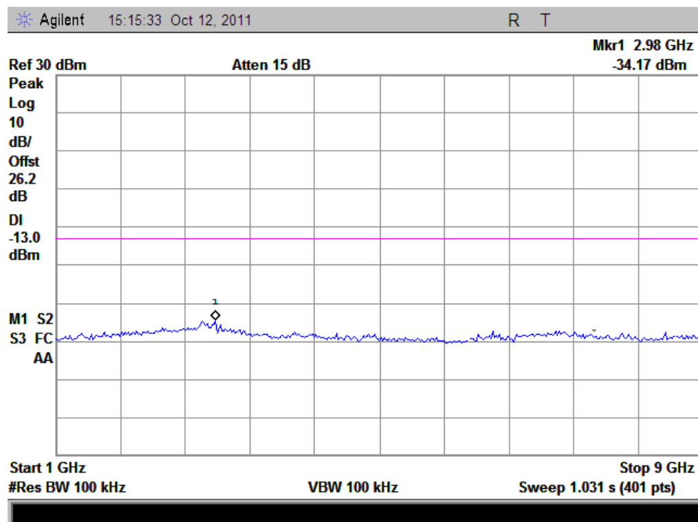
(Plot G3.1: HSDPA850MHz Channel = 4458, 1GHz to 9GHz)
