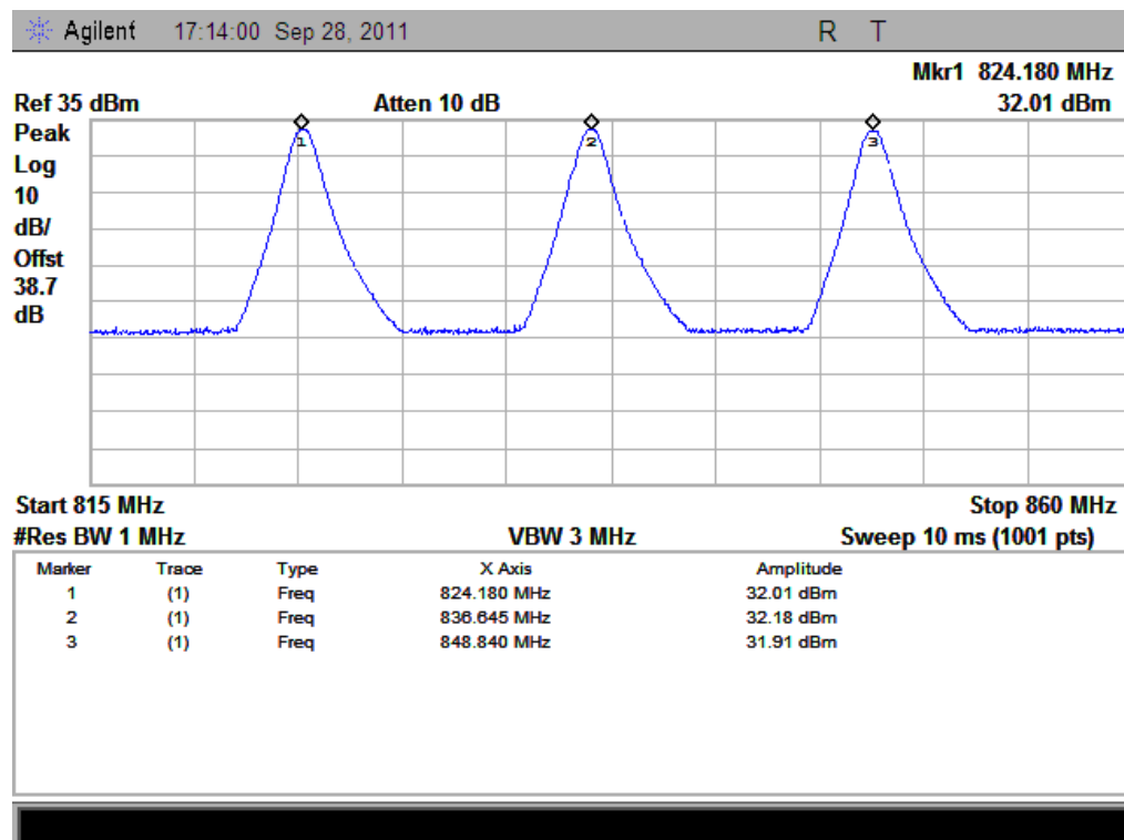
(Plot I: GPRS 850MHz Channel = 128, 190, 251)
