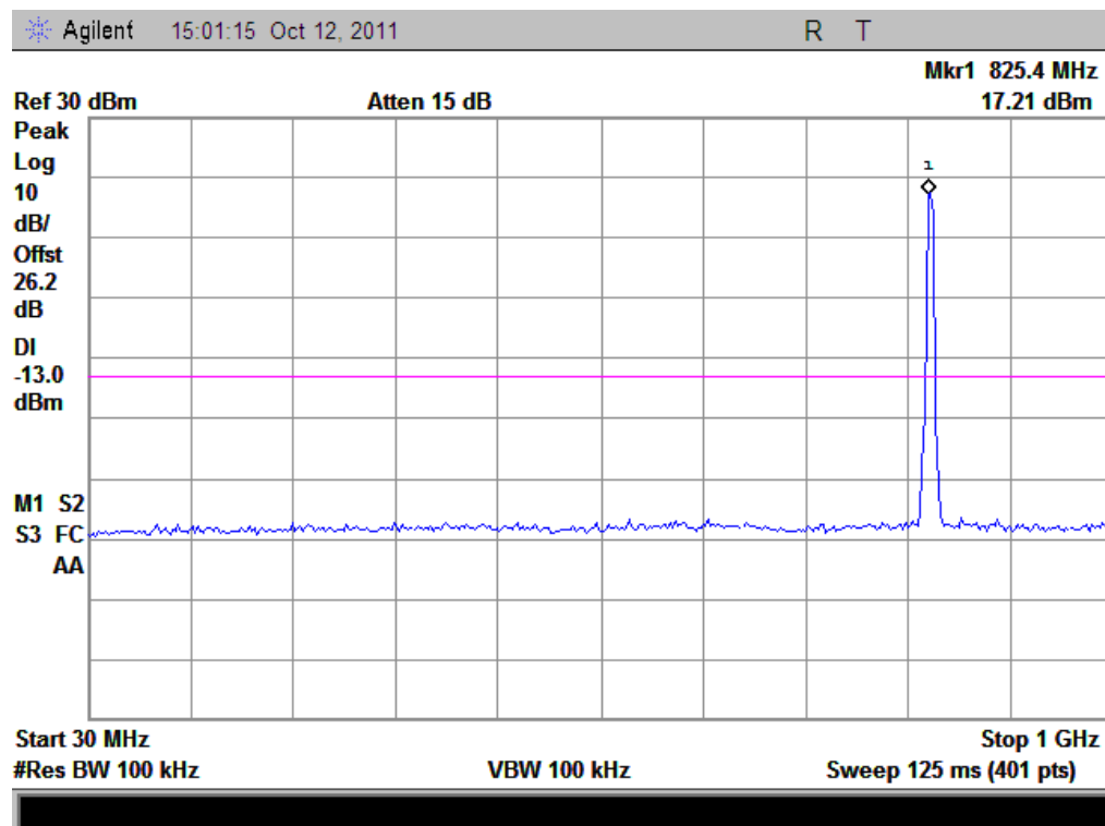
(Plot E1: WCDMA850MHz Channel = 4357, 30MHz to 1GHz)
