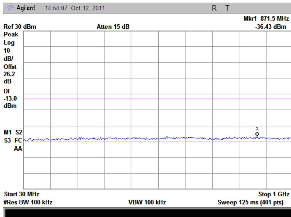
(Plot F3: WCDMA1900MHz Channel = 9938, 30MHz to 1GHz)
