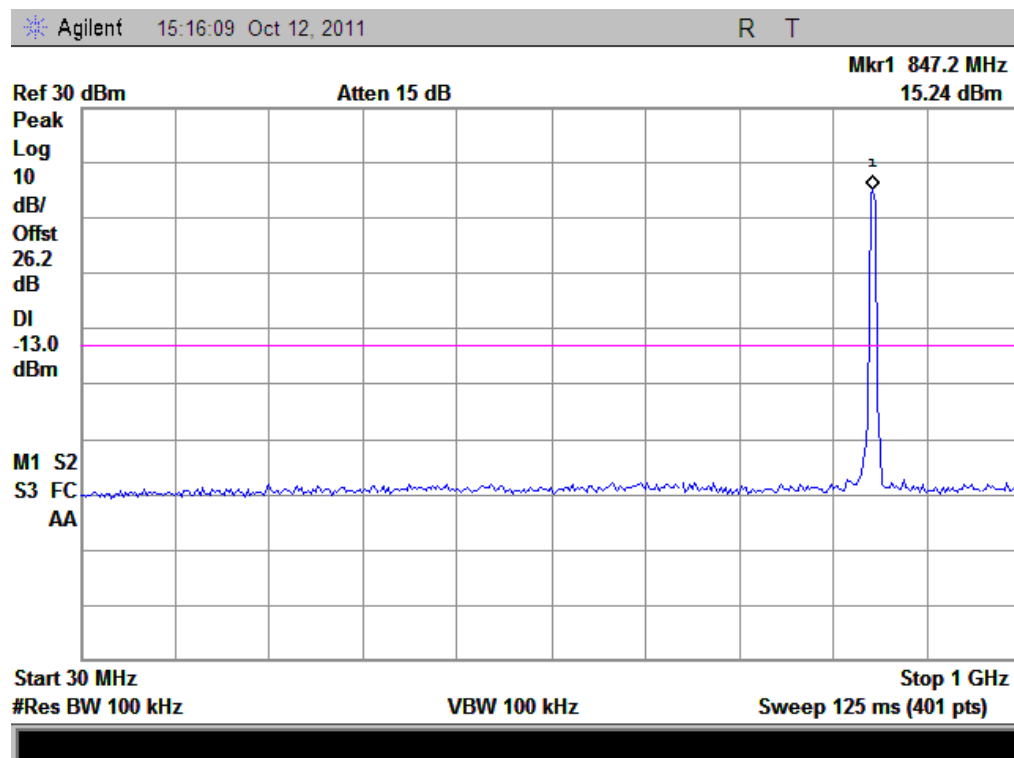
(Plot G3: HSDPA850MHz Channel = 4458, 30MHz to 1GHz)
