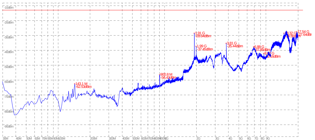
(Plot F.5: WCDMA 1900MHz Channel = 9938, Test Antenna Horizontal)
