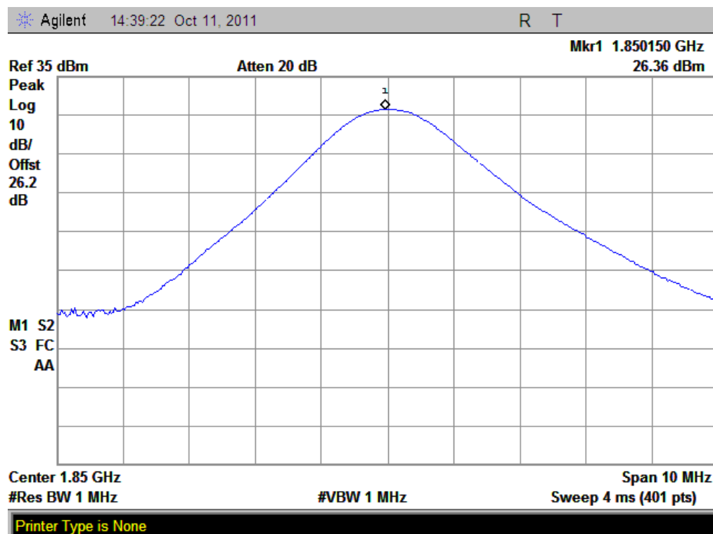
(Plot F1: GPRS 1900MHz Channel = 512)
