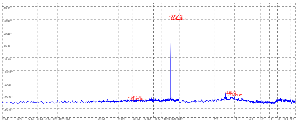
(Plot H: EDGE 850MHz Channel = 190, 30MHz to 10GHz)
