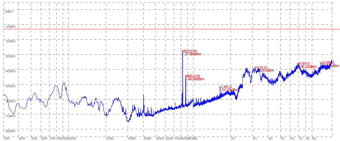
(Plot G.2: EGPRS 850MHz Channel = 128, Test Antenna Vertical)
