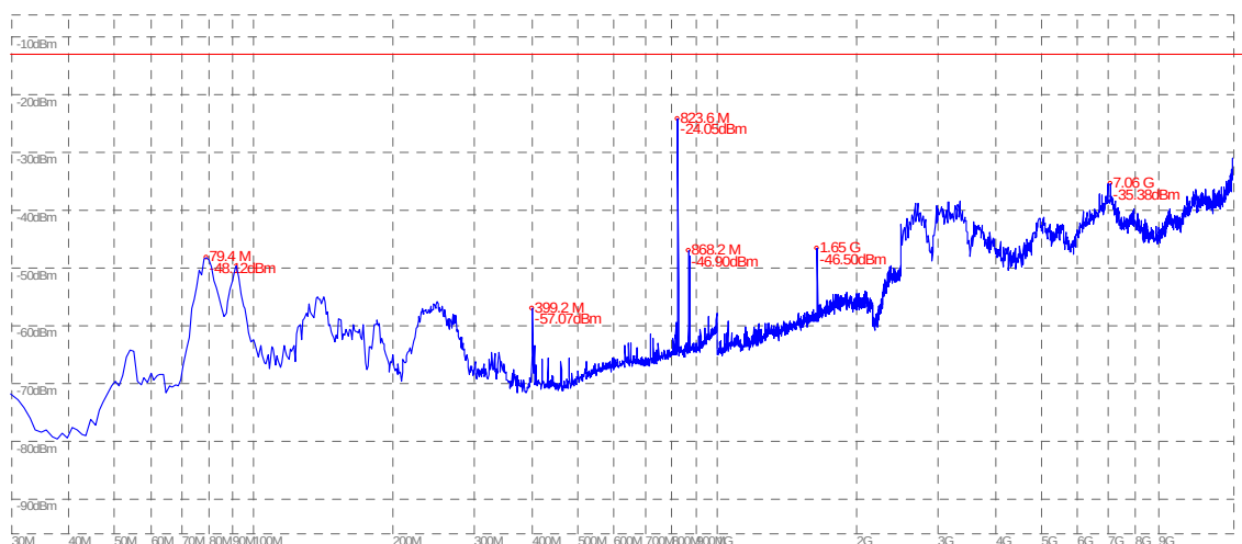
(Plot G.1: EGPRS 850MHz Channel = 128, Test Antenna Horizontal)
