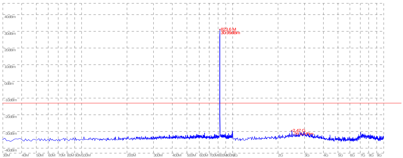
(Plot A1: GSM 850MHz Channel = 128, 30MHz to 10GHz)
