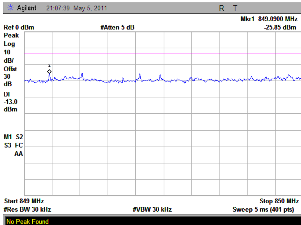
(Plot F: WCDMA 850 Channel = 4458)
