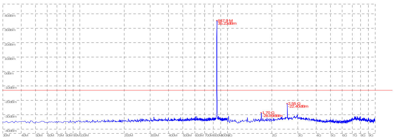
(Plot A3: GSM 850MHz Channel = 251, 30MHz to 10GHz)
