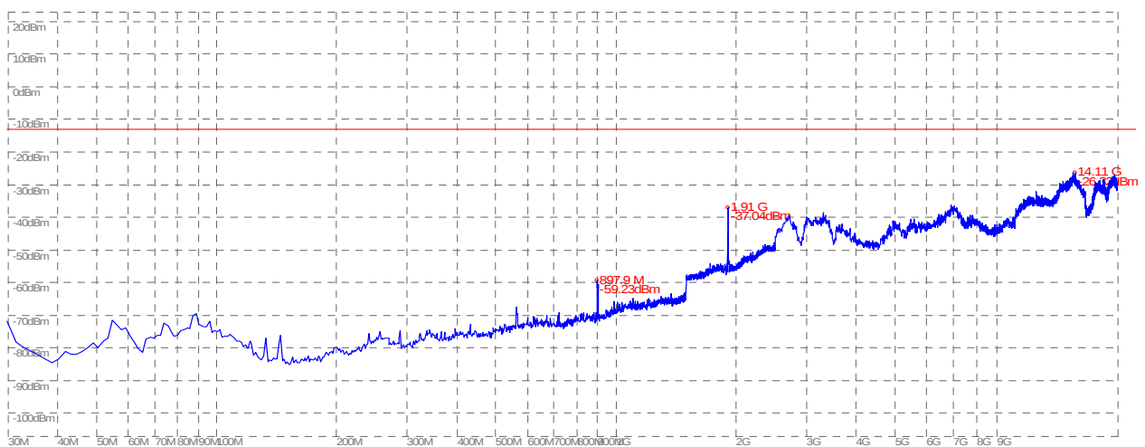
(Plot D.5: WCDMA 1900MHz Channel = 9938, Test Antenna Horizontal)
