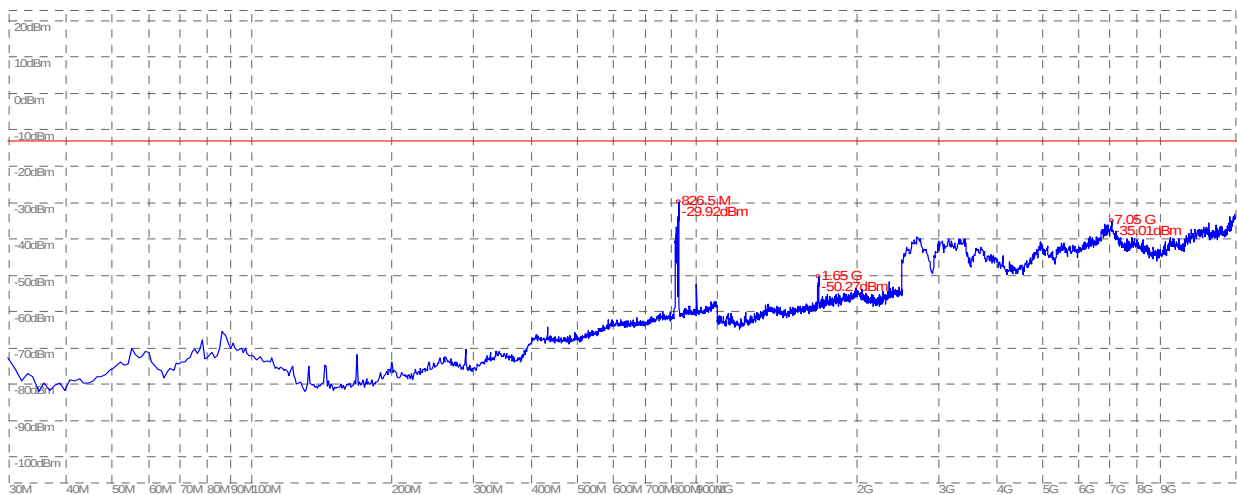
(Plot C.1: WCDMA 850MHz Channel = 4357, Test Antenna Horizontal)
