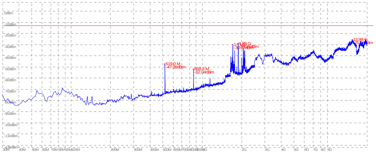
(Plot B.3: GSM 1900MHz Channel = 661, Test Antenna Horizontal)
