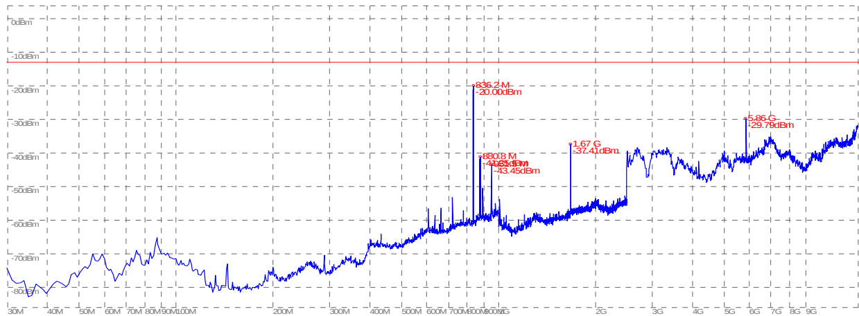
(Plot A.3: GSM 850MHz Channel = 190, Test Antenna Horizontal)
