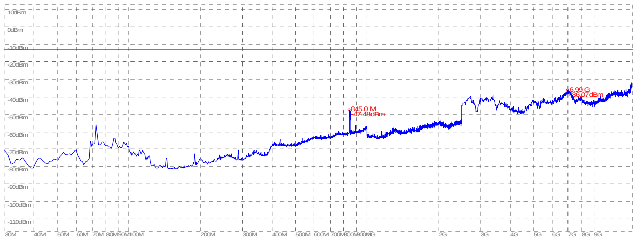
(Plot C.6: WCDMA 850MHz Channel = 4458, Test Antenna Vertical)
