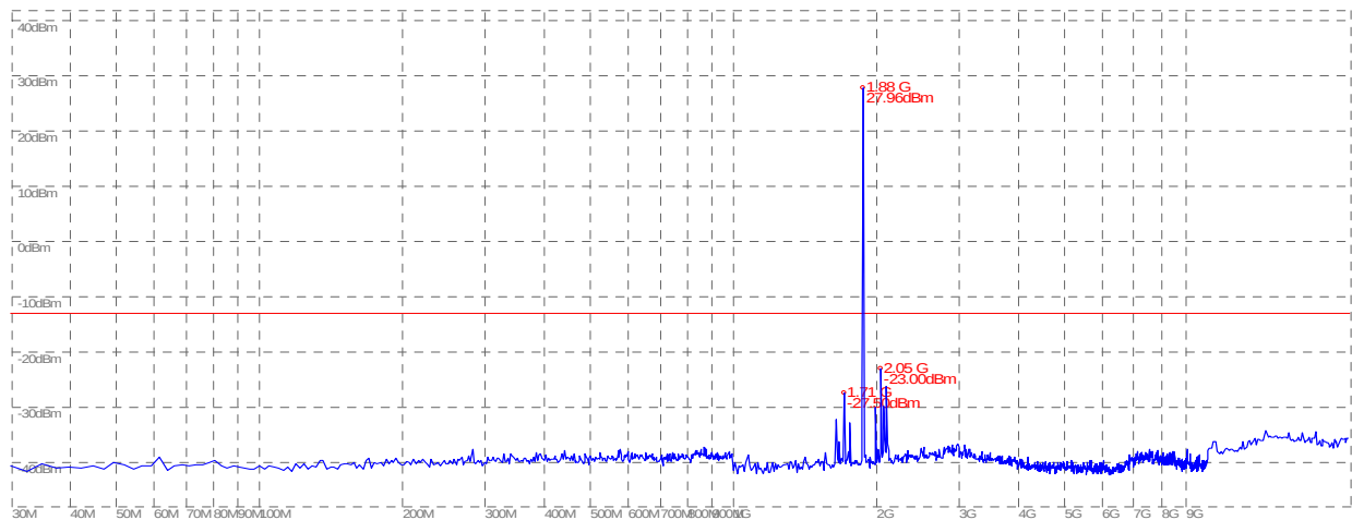
(Plot B2: GSM 1900MHz Channel = 661, 30MHz to 20GHz)
