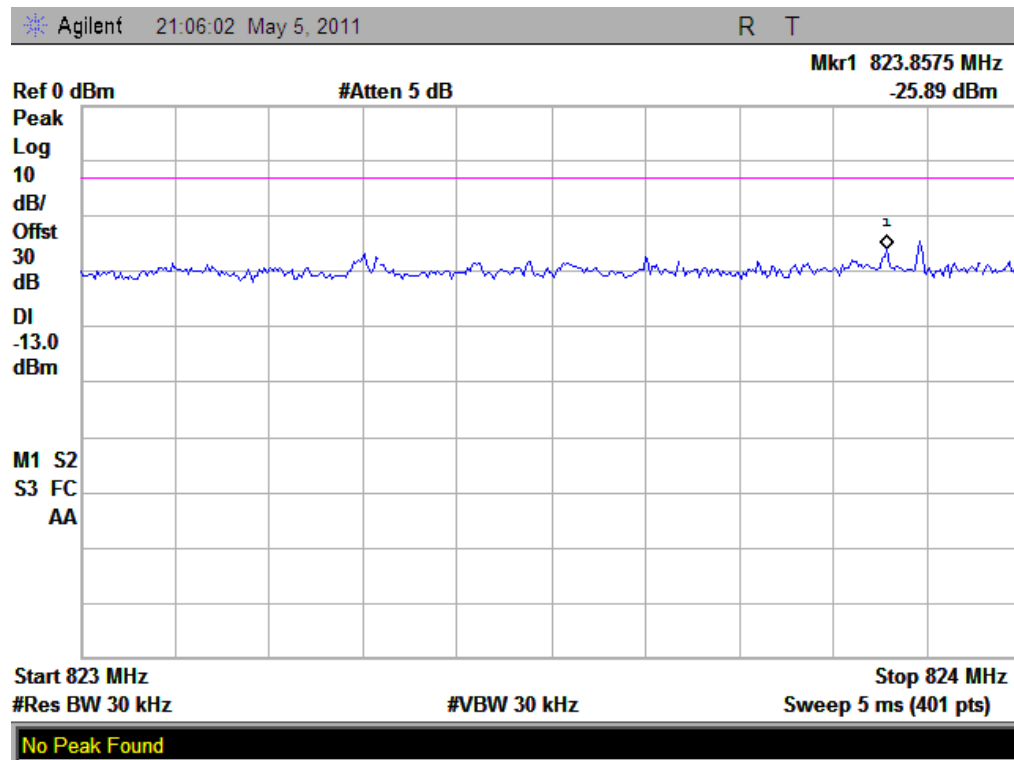
(Plot E: WCDMA 850 Channel = 4357)
