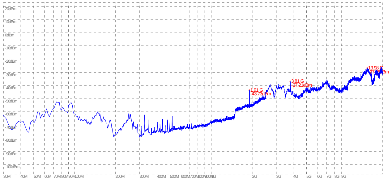
(Plot D.6: WCDMA 1900MHz Channel = 9938, Test Antenna Vertical)
