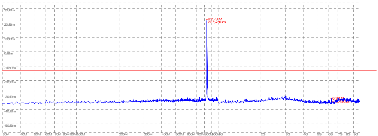
(Plot C2: WCDMA 850MHz Channel = 4400, 30MHz to 10GHz)
