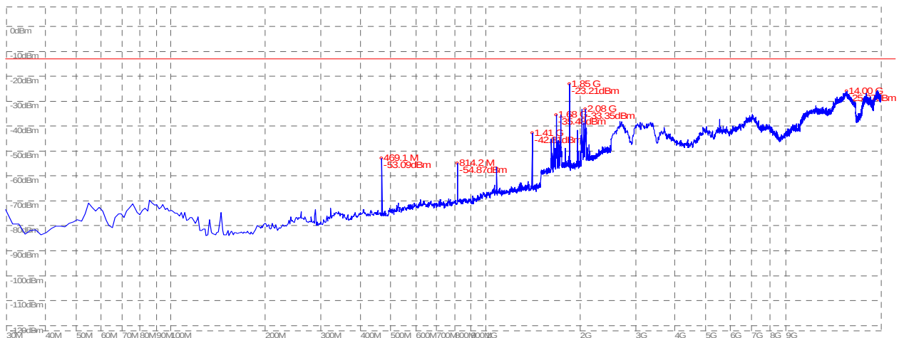
(Plot B.1: GSM 1900MHz Channel = 512, Test Antenna Horizontal)
