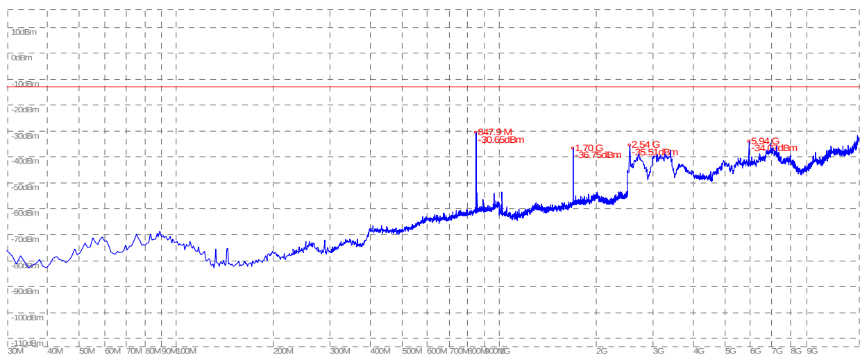
(Plot A.5: GSM 850MHz Channel = 251, Test Antenna Horizontal)
