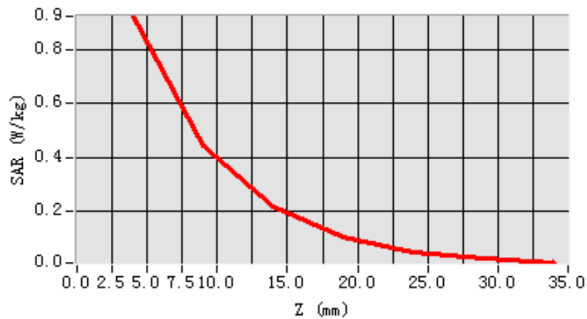
SAR, Z Axis Scan (X = -8, Y = 11)
