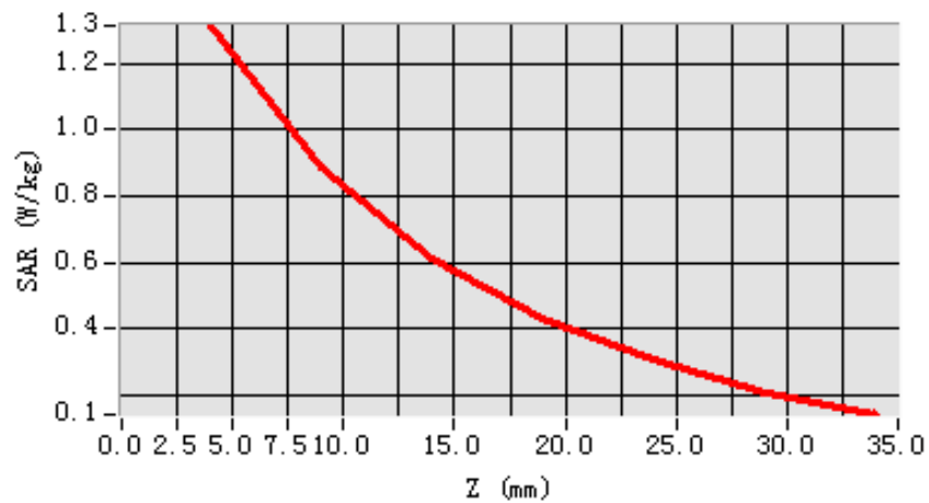
SAR, Z Axis Scan (X = -31, Y = -11)
