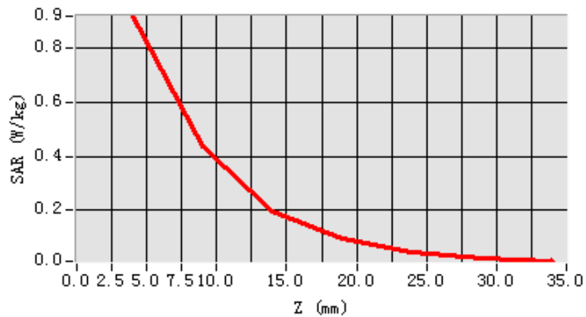
SAR, Z Axis Scan (X = -2, Y = 41)
