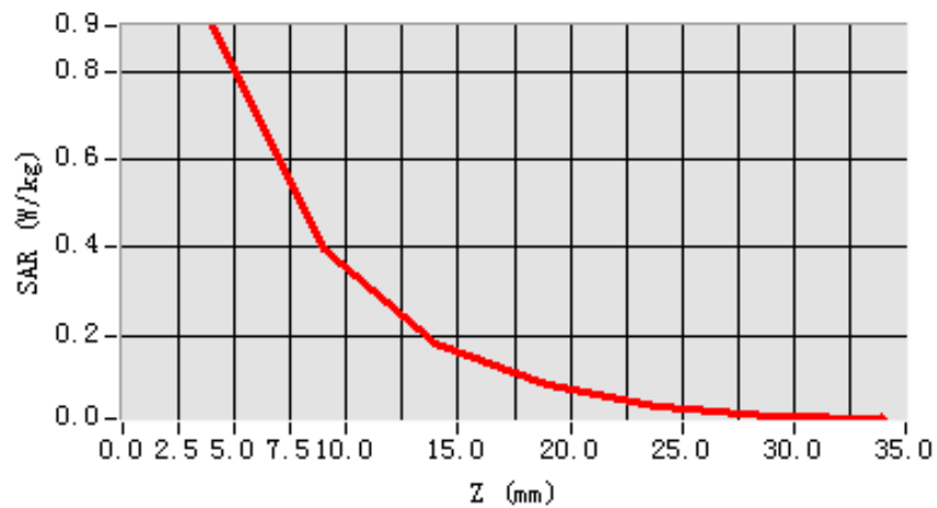
SAR, Z Axis Scan (X = -16, Y = 11)
