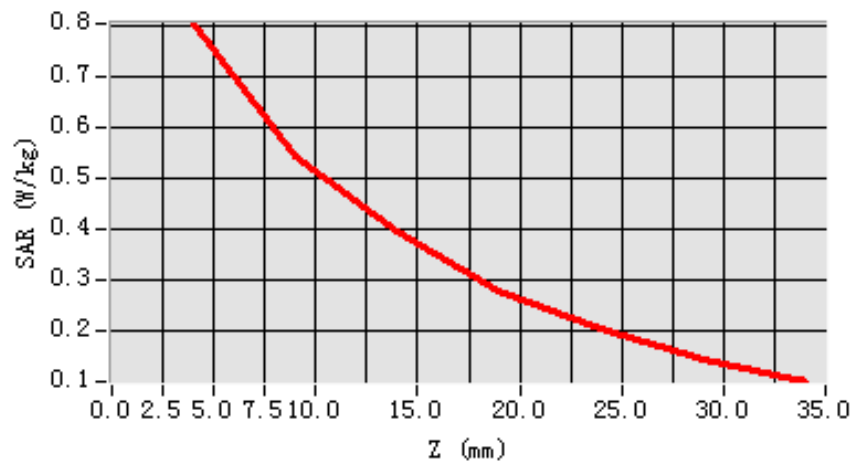
SAR, Z Axis Scan (X = -24, Y = -13)
