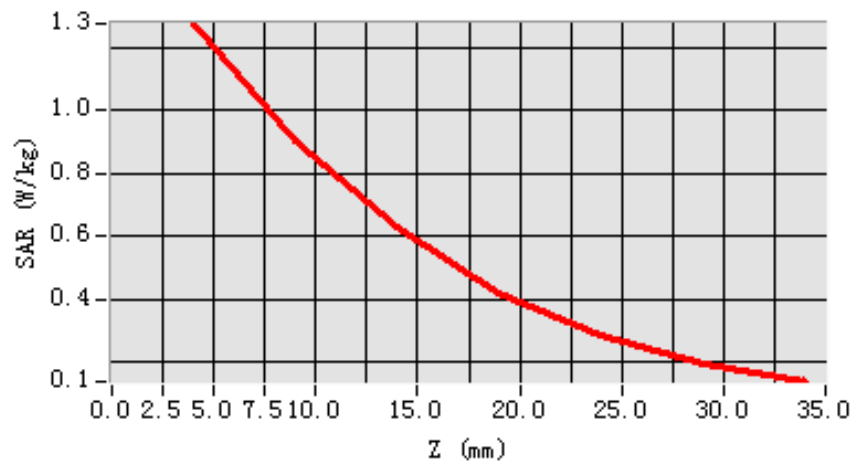
SAR, Z Axis Scan (X = -30, Y = -14)
