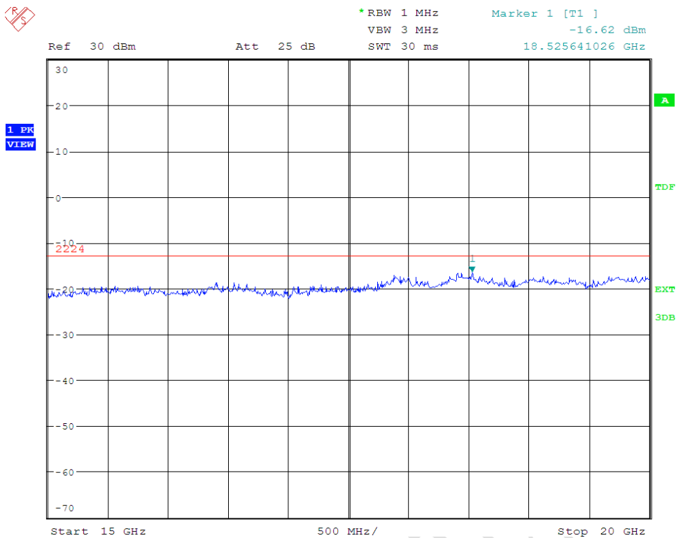
Channel 9400 for 1900MHz – 15GHz to 20GHz
