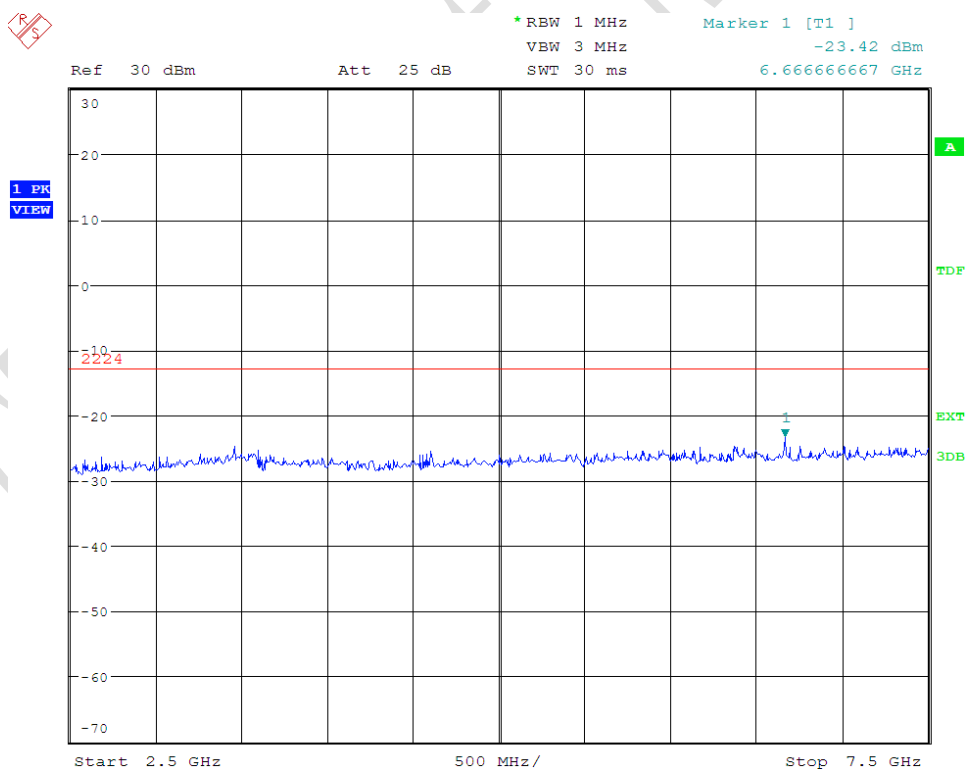
Channel 9400 for 1900MHz – 2.5GHz to 7.5GHz
