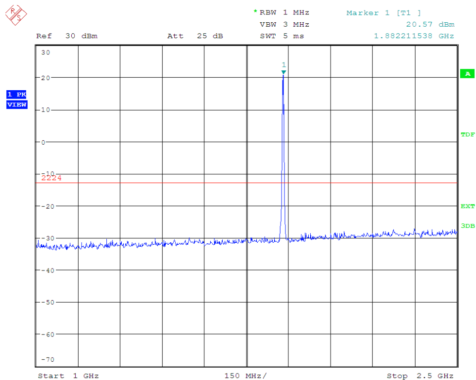
Channel 9400 for 1900MHz – 1GHz to 2.5GHz
