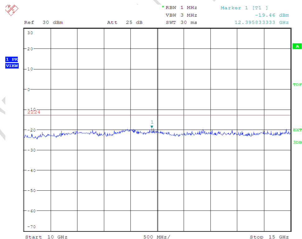
Channel 9400 for 1900MHz – 10GHz to 15GHz
