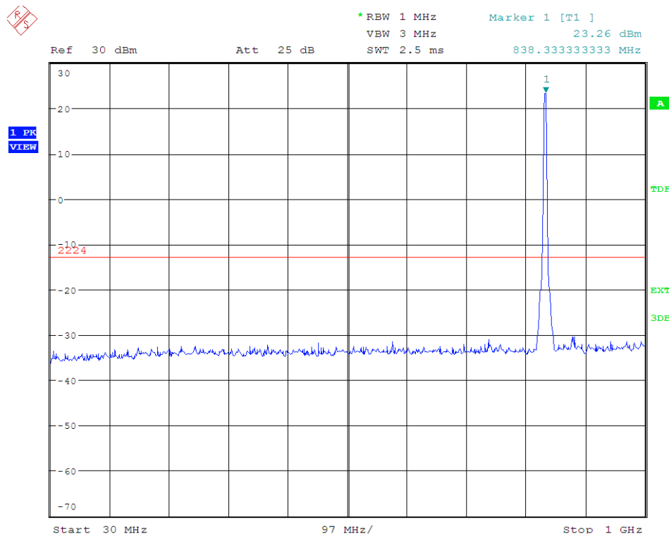
Channel 4183 for 850MHz – 30MHz to 1GHz
