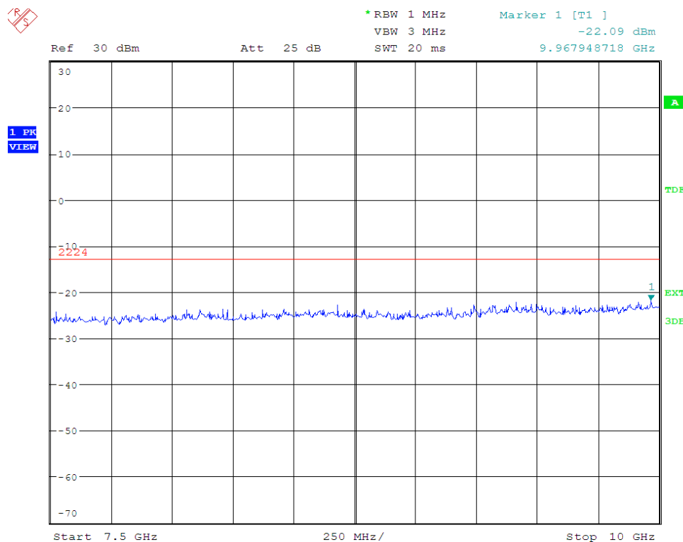
Channel 9400 for 1900MHz – 7.5GHz to 10GHz
