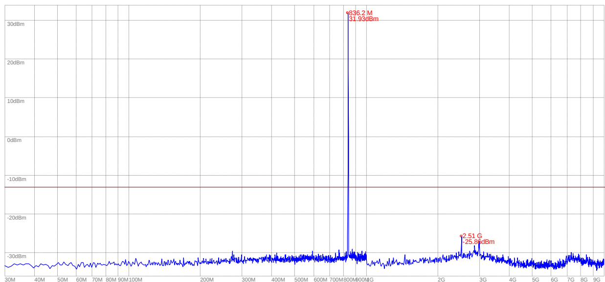
(Plot H: EDGE 850MHz Channel = 190, 30MHz to 10GHz)
