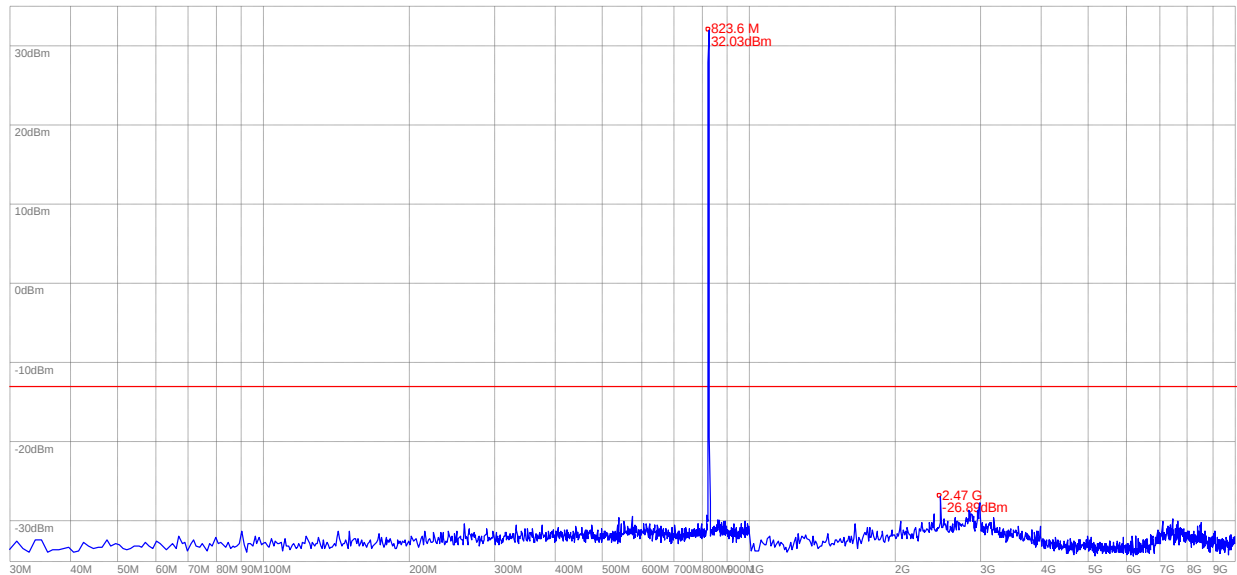
(Plot G: EDGE 850MHz Channel = 128, 30MHz to 10GHz)
