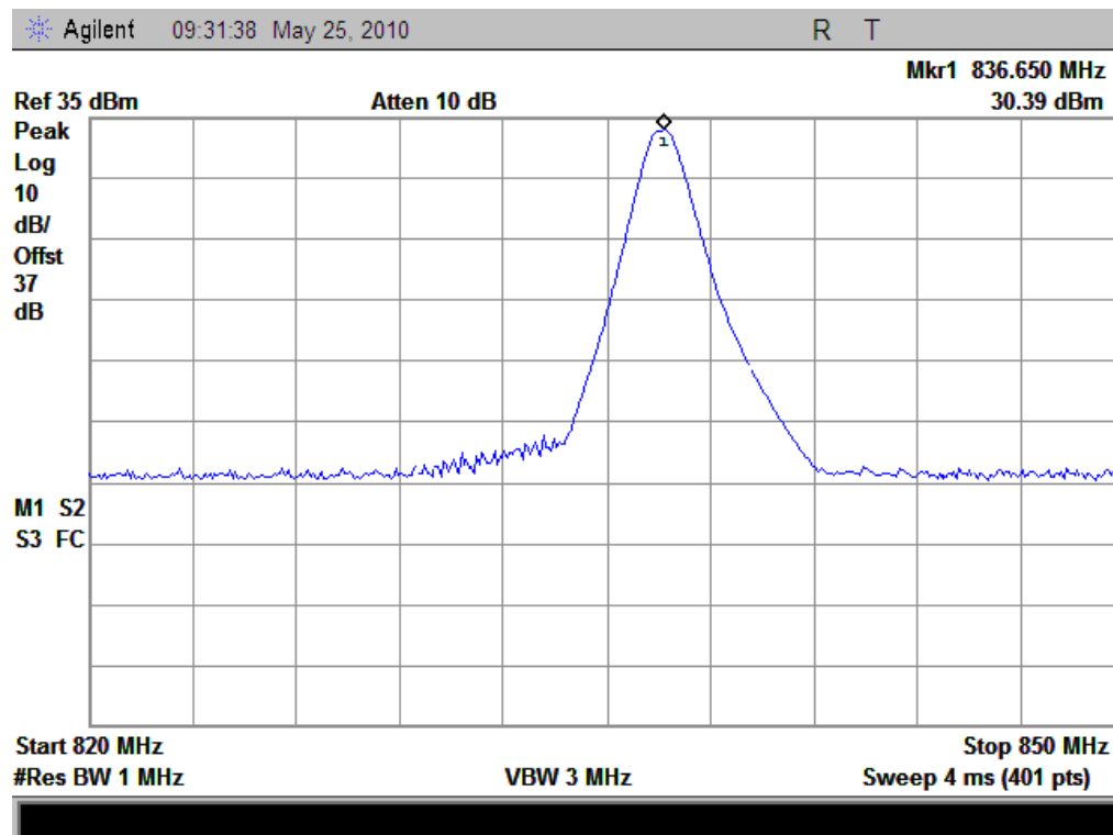
(Plot H: GPRS-2TX 850MHz Channel =190)
