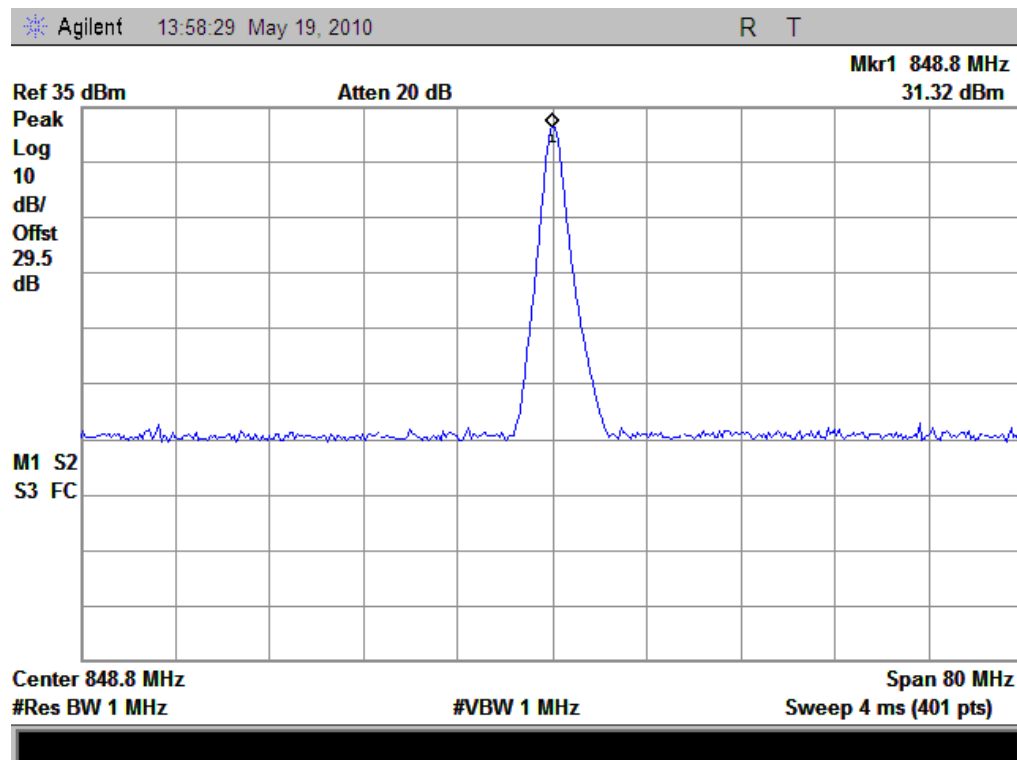
(Plot G: GPRS-2TX 850MHz Channel = 251)
