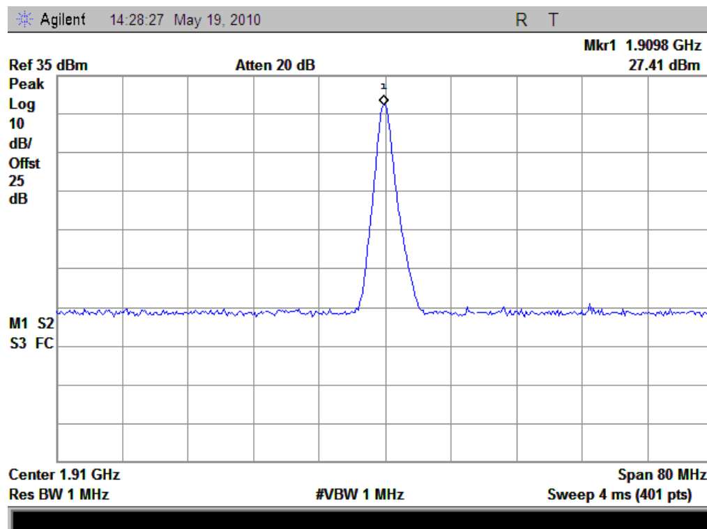
(Plot G: GPRS-2TX 1900MHz Channel = 810)
