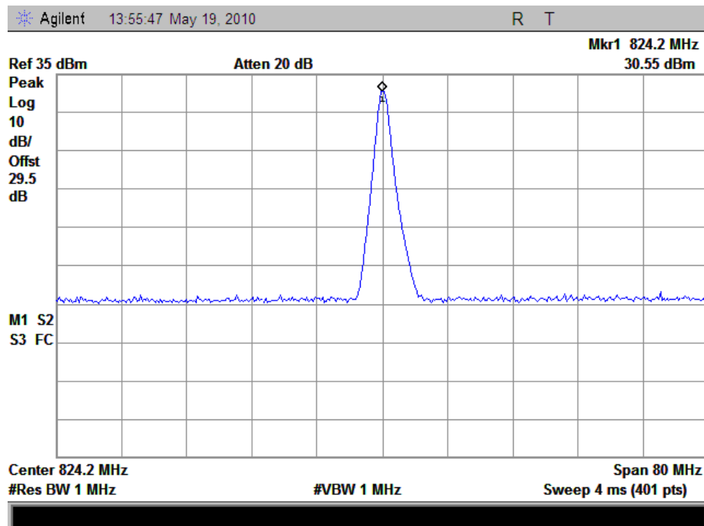
(Plot G: GPRS-2TX 850MHz Channel = 128)
