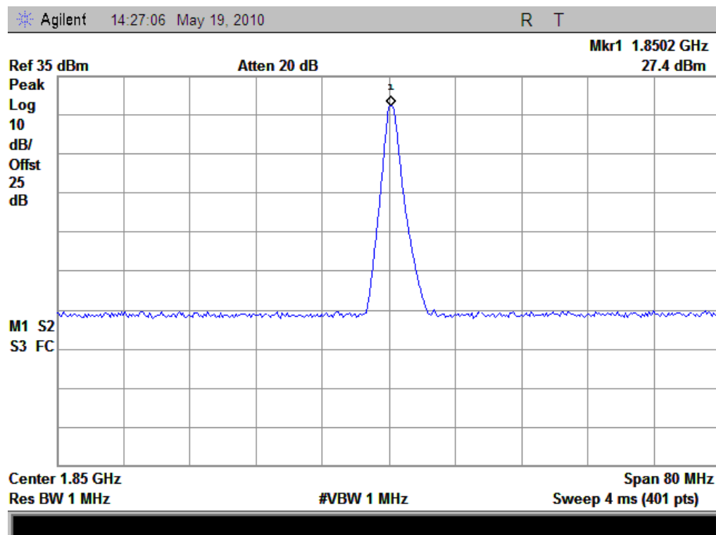
(Plot G: GPRS-2TX 1900MHz Channel = 512)
