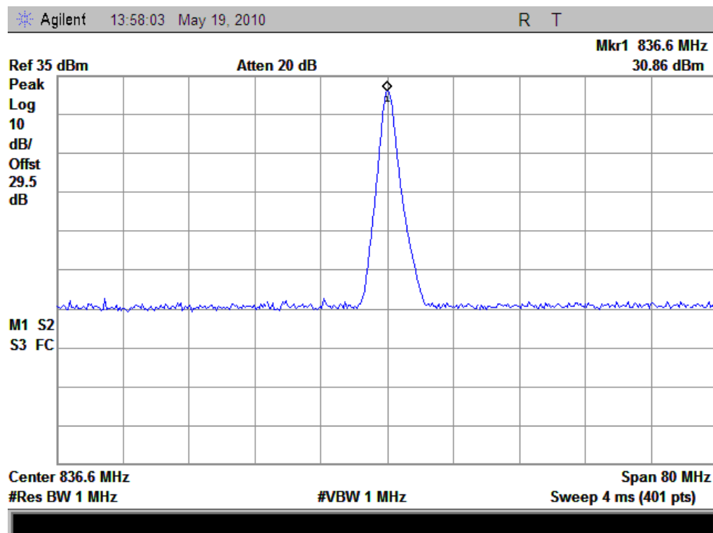
(Plot G: GPRS-2TX 850MHz Channel = 190)
