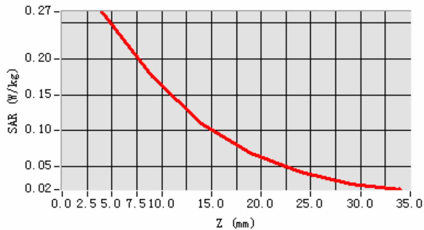
SAR, Z Axis Scan (X = -19, Y = 0)
