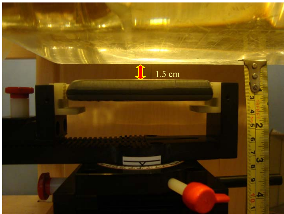
Body-worn Back Setup Photo (GPRS Model)
