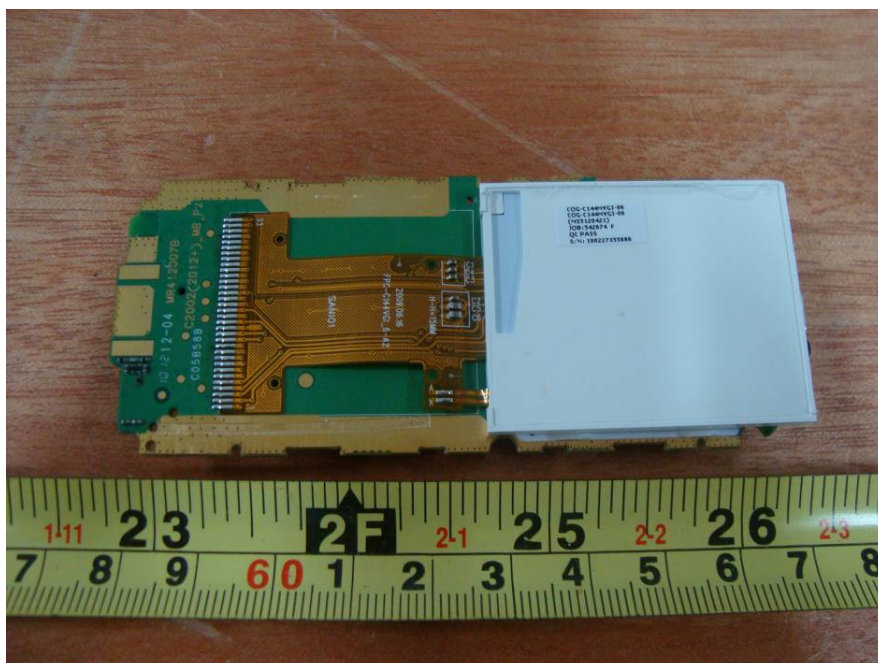
EUT – Main Board without LCD Panel Top View
