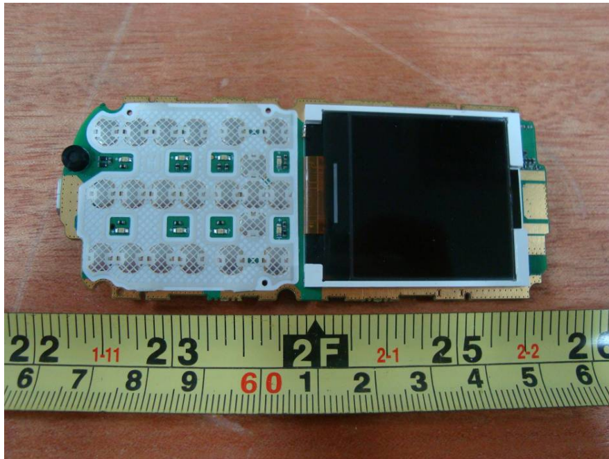
EUT – Main Board with LCD Panel Top View
