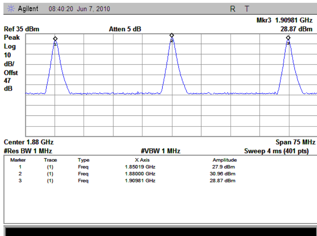
(Plot B: GPRS 1900MHz Channel = 512, 661, 810)
