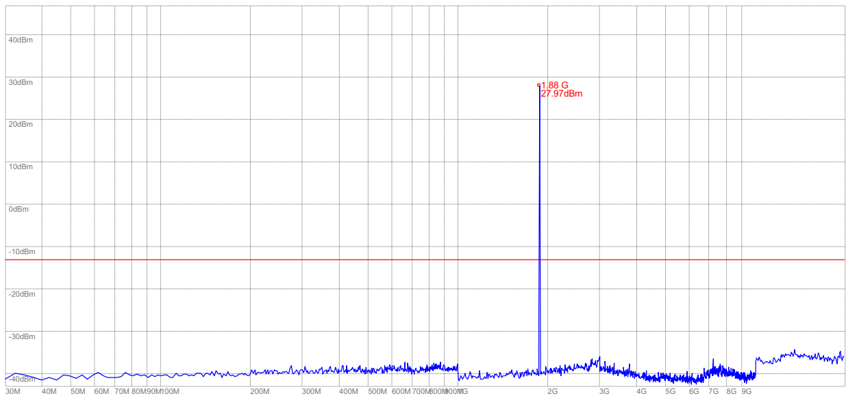
(Plot B: GSM 1900MHz Channel = 661, 30MHz to 20GHz)
