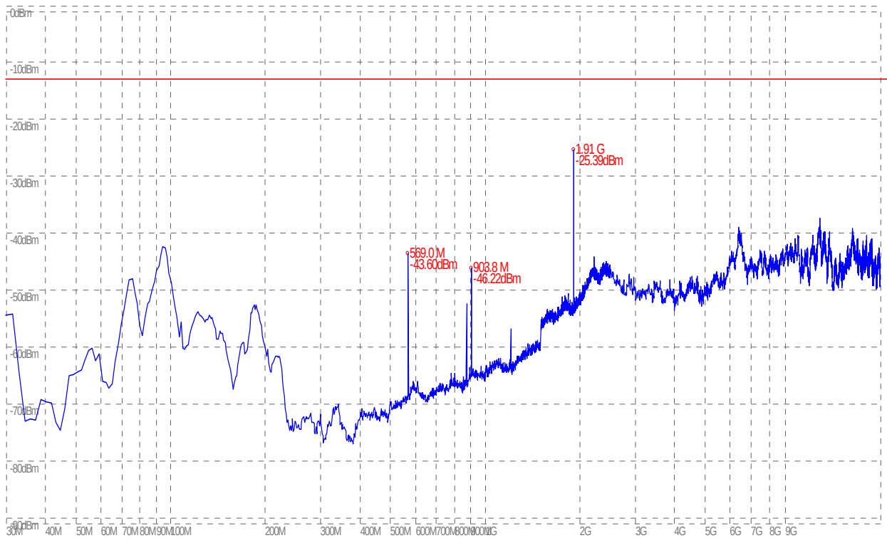
(PlotB.6: GSM 1900MHz Channel = 810, Test Antenna Vertical)
