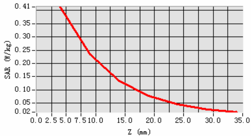
SAR, Z Axis Scan (X = 16, Y = 38)
