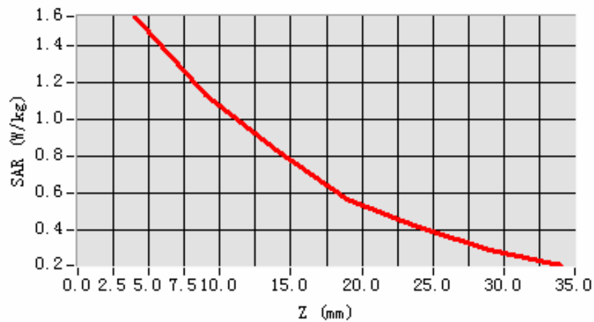
SAR, Z Axis Scan (X = -28, Y = -18)
