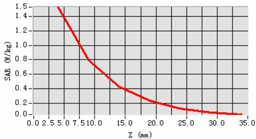
SAR, Z Axis Scan (X = -19, Y = 11)
