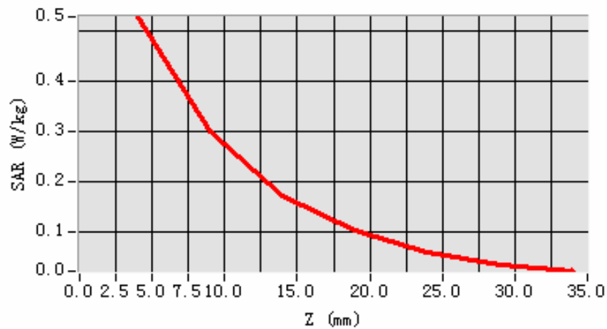
SAR, Z Axis Scan (X = 17, Y = 31)
