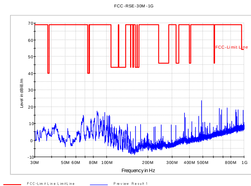
Fig. 45 Radiated Spurious Emission (802.11g, Ch1, 30 MHz-1 GHz)
