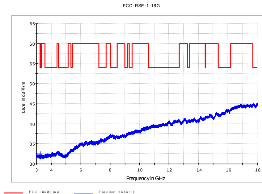
Fig. 53 Radiated Spurious Emission (802.11g, Ch11, 3 GHz-18 GHz)
