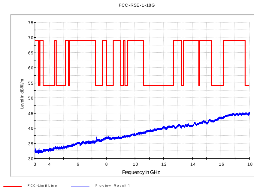
Fig. 41 Radiated Spurious Emission (802.11b, Ch6, 3 GHz-18 GHz)
