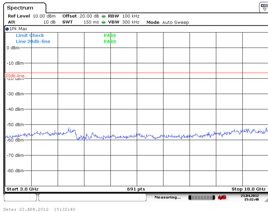
Fig. 25 Conducted Spurious Emission (802.11b, Ch11, 3 GHz-18 GHz)
