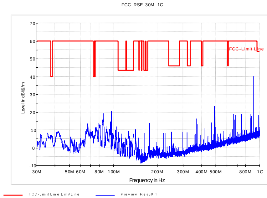
Fig. 48 Radiated Spurious Emission (802.11g, Ch6, 30 MHz-1 GHz)
