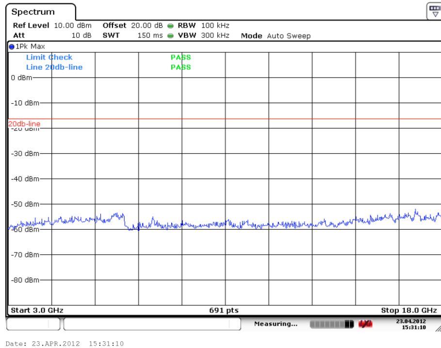
Fig. 19 Conducted Spurious Emission (802.11b, Ch1, 3 GHz-18 GHz)
