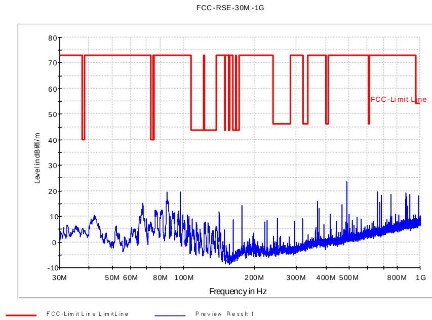
Fig. 42 Radiated Spurious Emission (802.11b, Ch11, 30 MHz-1 GHz)
