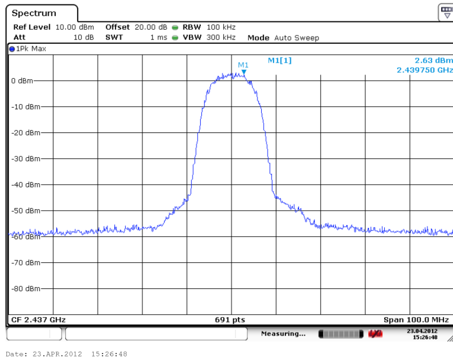
Fig. 20 Conducted Spurious Emission (802.11b, Ch6, Center Frequency)
