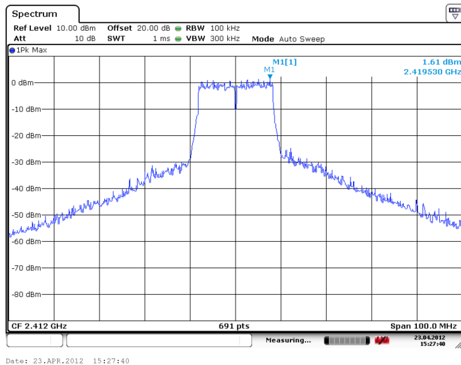
Fig. 26 Conducted Spurious Emission (802.11g, Ch1, Center Frequency)
