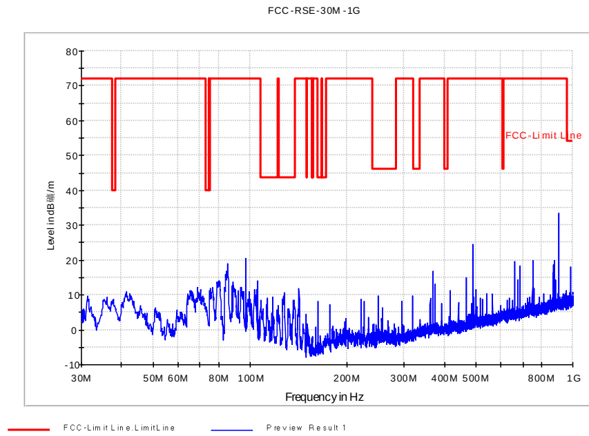
Fig. 36 Radiated Spurious Emission (802.11b, Ch1, 30 MHz-1 GHz)
