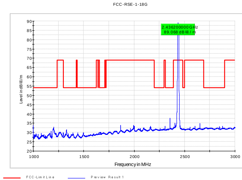
Fig. 40 Radiated Spurious Emission (802.11b, Ch6, 1 GHz-3 GHz)
