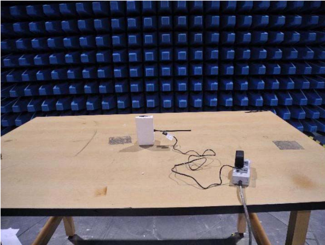
FCC Part 22H/24E Radiated Emission above 1GHz
