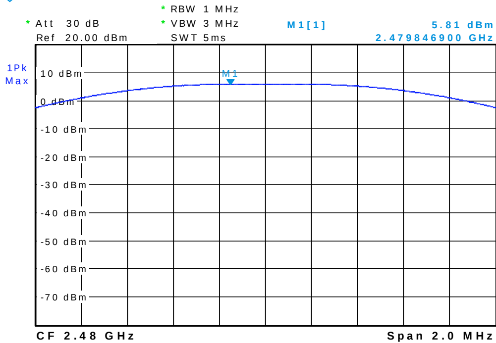
Measurement Results (Modulation: 8DQPSK)
