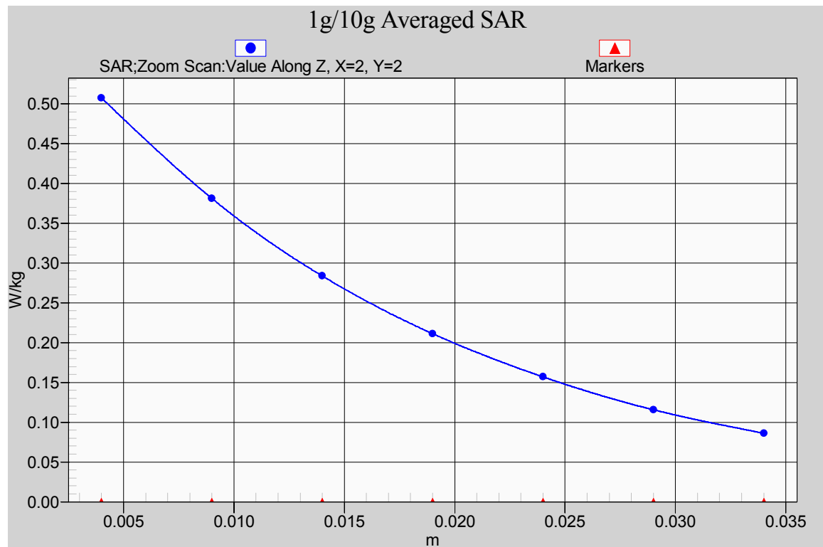
Fig. 3-1 Z-Scan at power reference point (850 MHz CH251)
