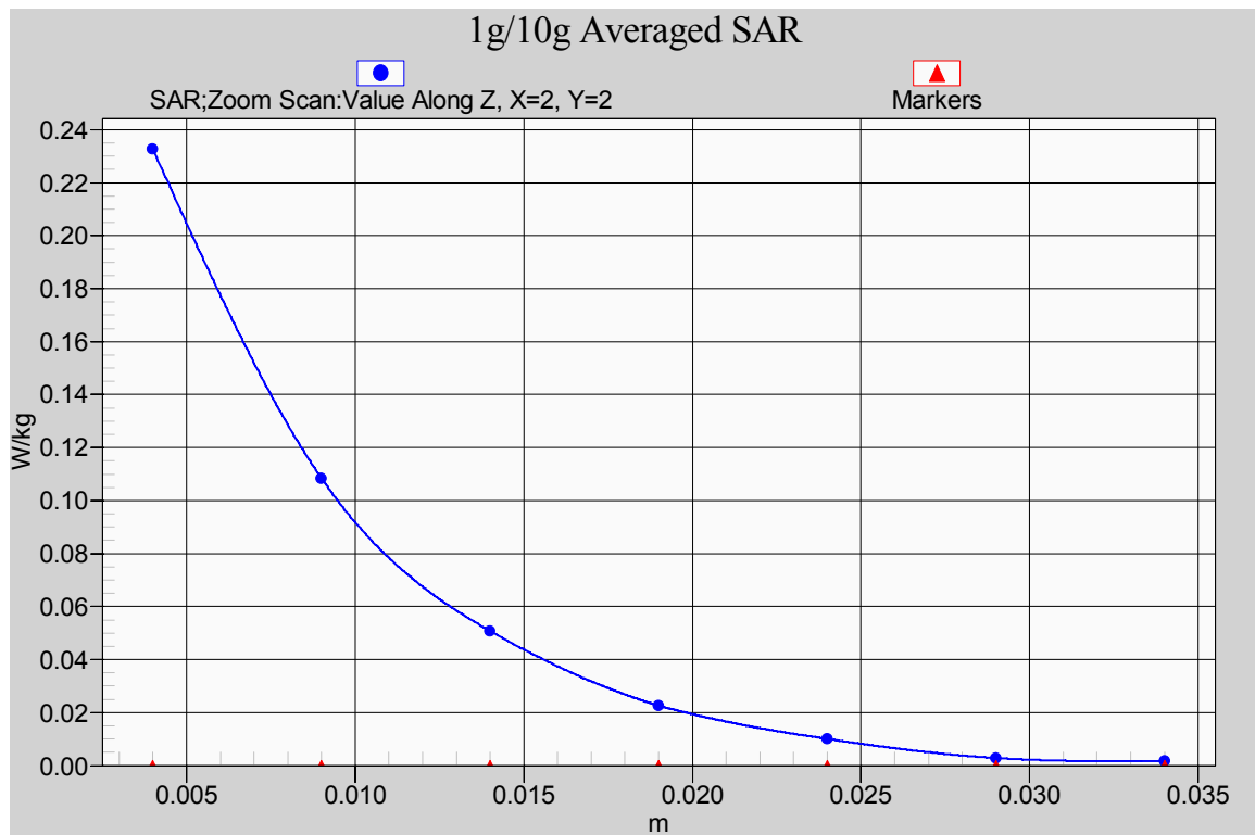
Fig. 25-1 Z-Scan at power reference point (2450 MHz CH1)
