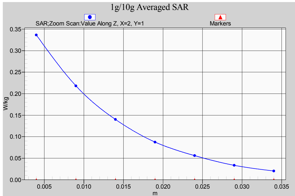
Fig. 19-1 Z-Scan at power reference point (1900 MHz CH810)
