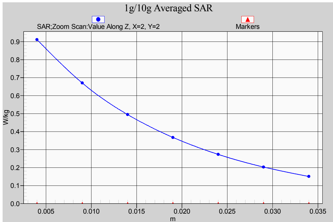
Fig. 8-1 Z-Scan at power reference point (850 MHz CH251)
