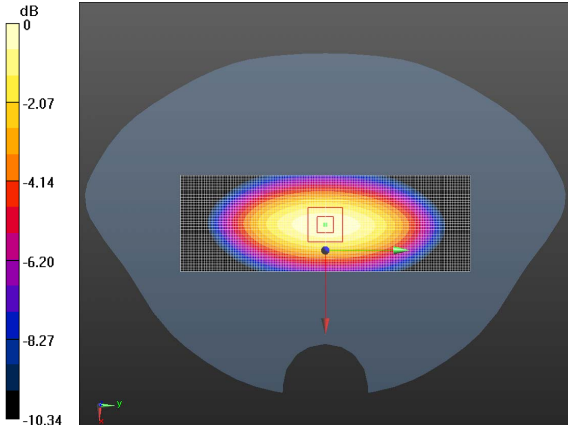
Fig.B.1 validation 835MHz 250mW
