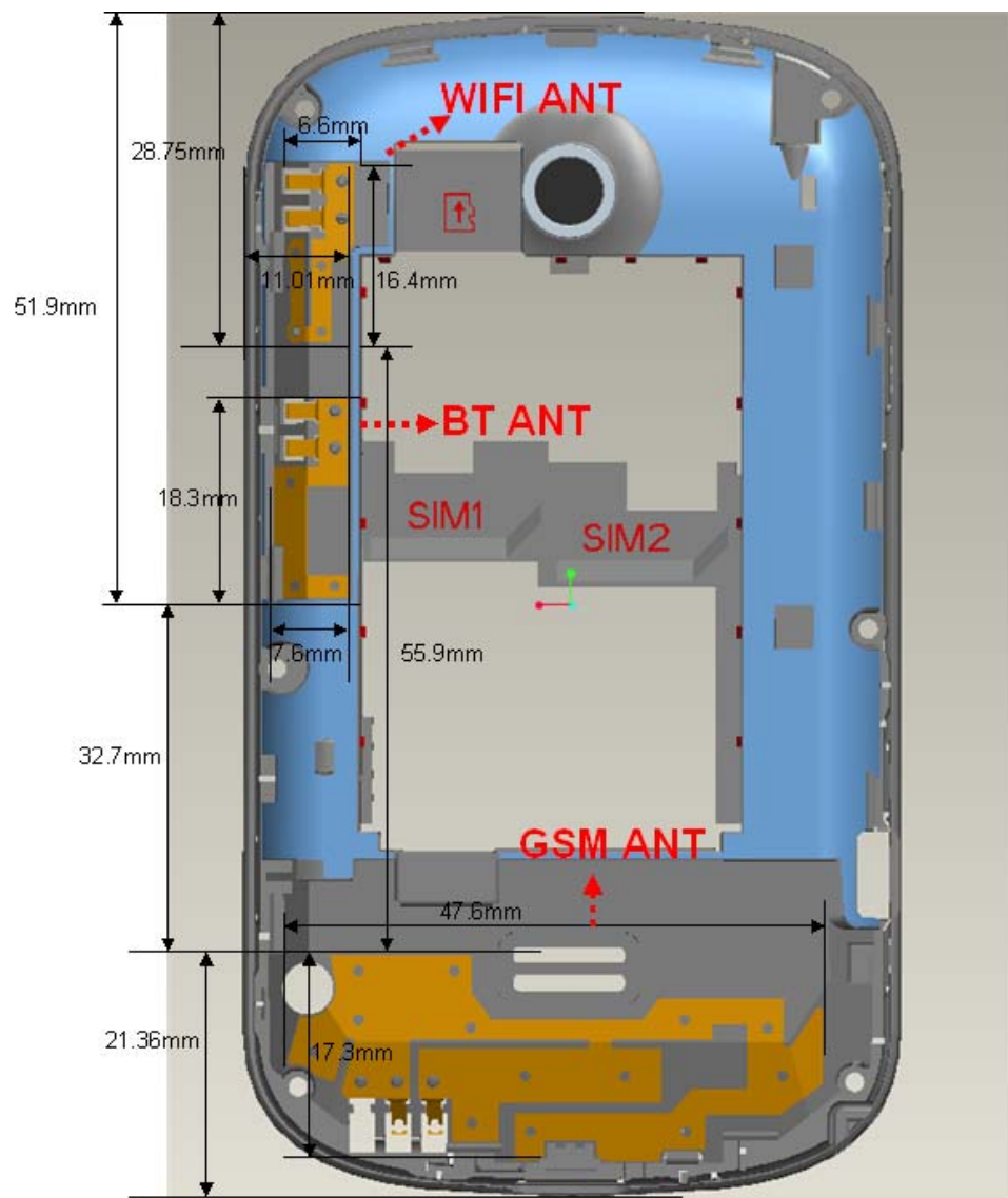
Picture 11.1 Antenna Locations
