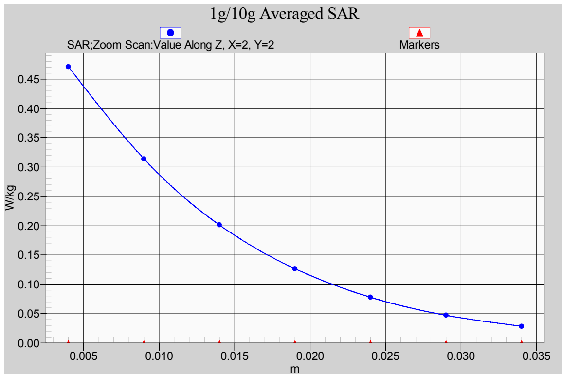
Fig. 14-1 Z-Scan at power reference point (1900 MHz CH810)
