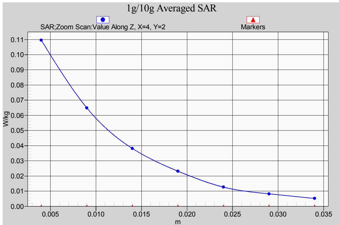
Fig. 33-1 Z-Scan at power reference point (2450 MHz CH11)
