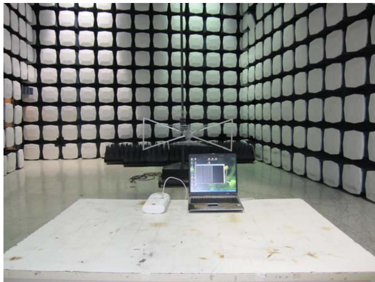
Radiated Emission Test Photos
