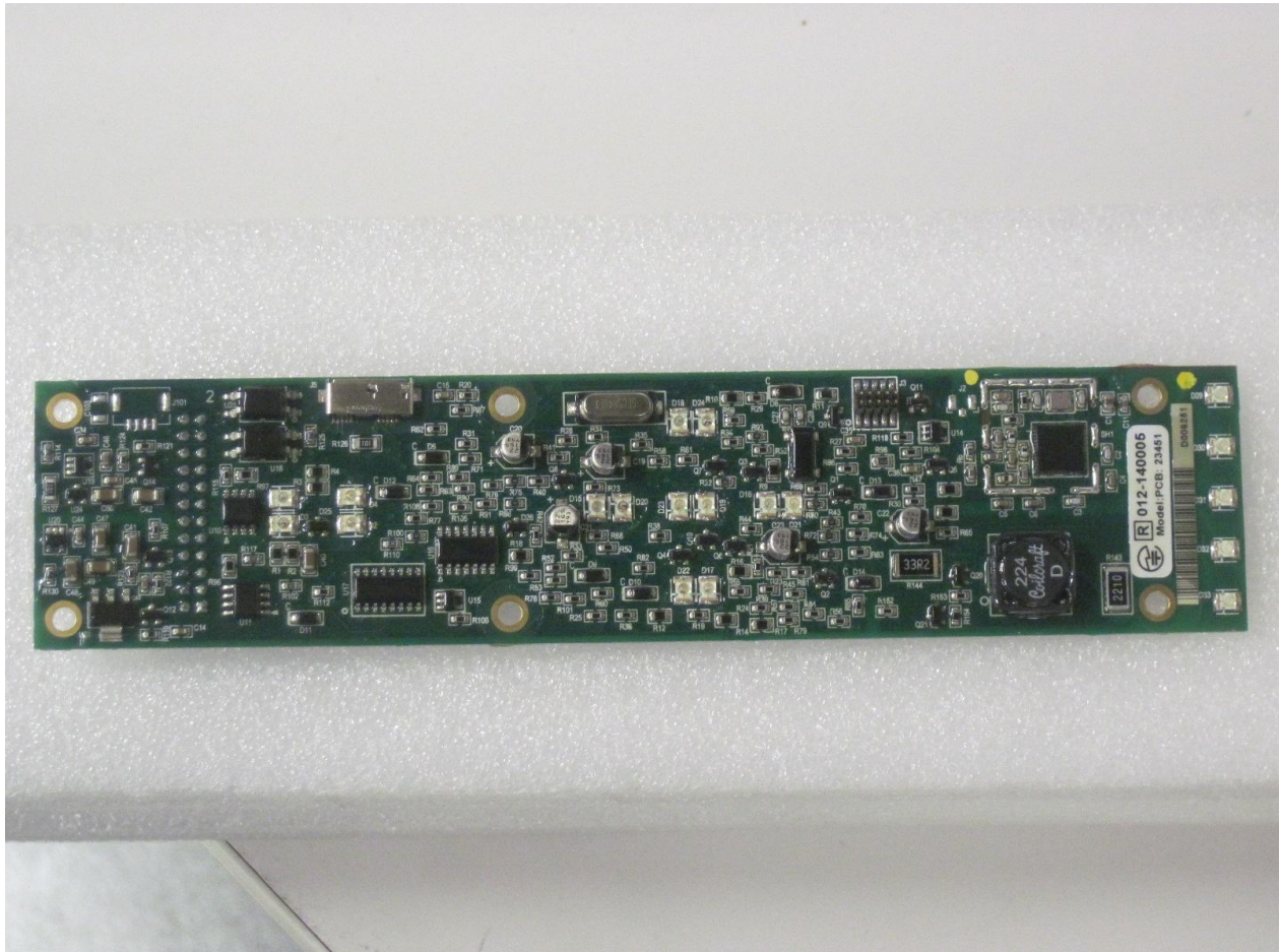
PCB, Model #23451-00001 (top side)
