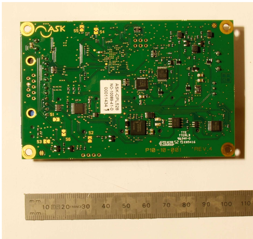
CLESS reader board Bot
