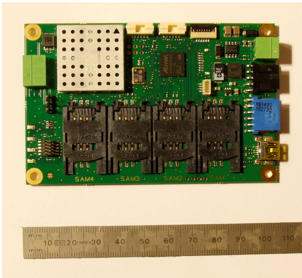
CLESS reader board Top with shielding
