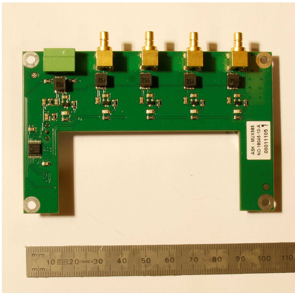
Switch antenna board Top
