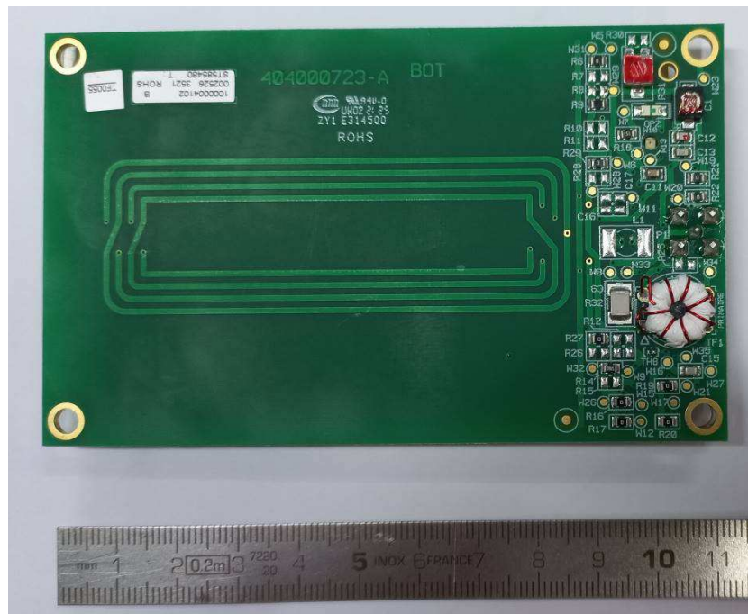
Unstacker antenna Top (ELM_1000004108)
