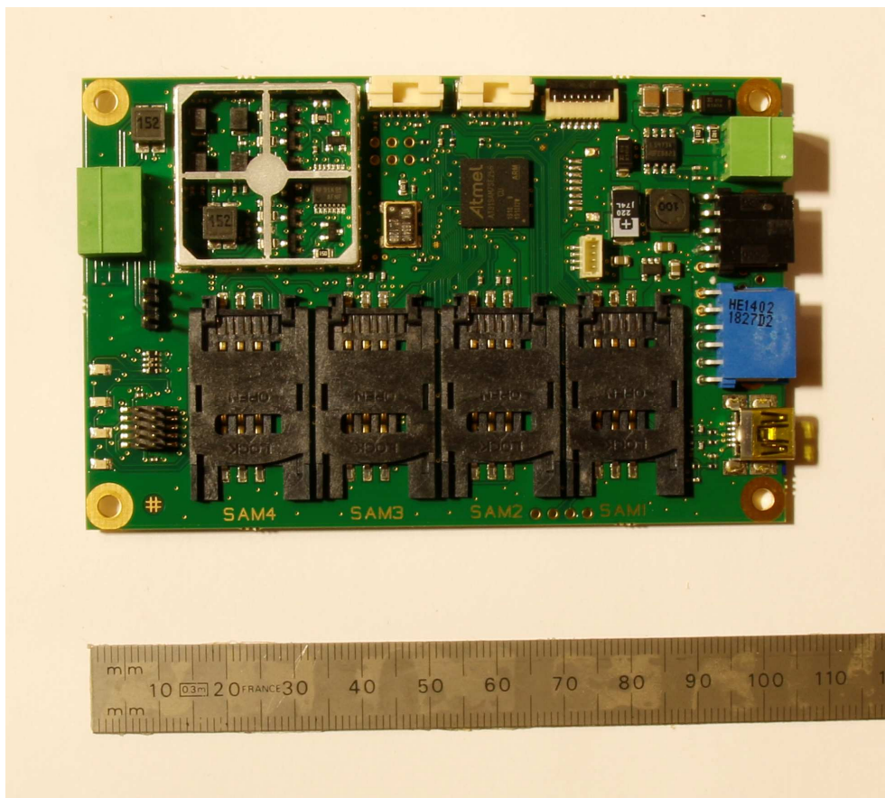
CLESS reader board Top without shielding
