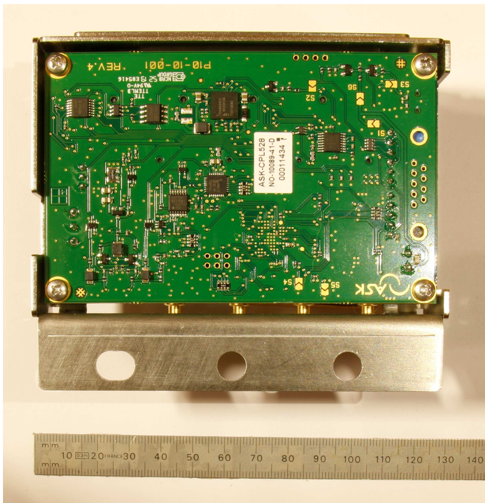
CLESS reader Bottom view
