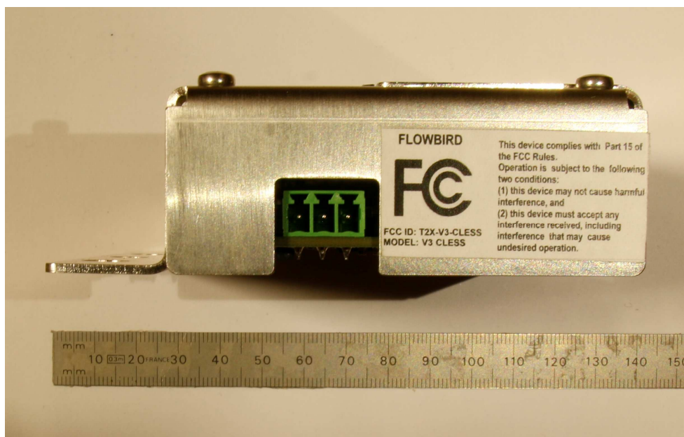
CLESS reader Side view
