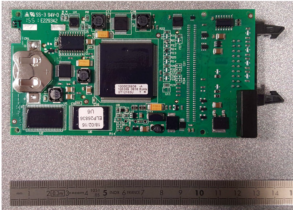
Card reader board Top
