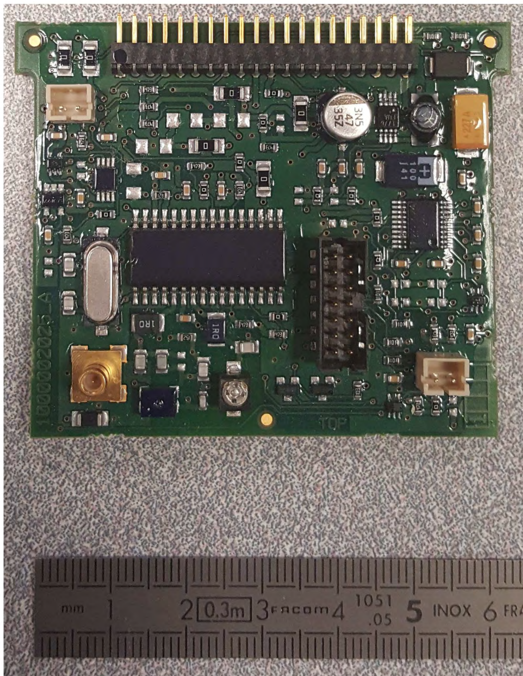
Cless board Top
