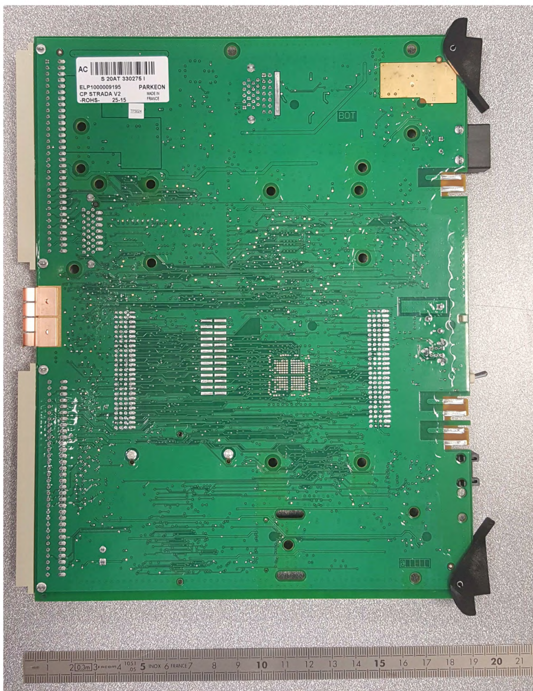
Main board Bot
