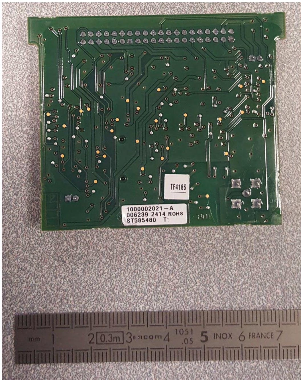
Cless board Bot
