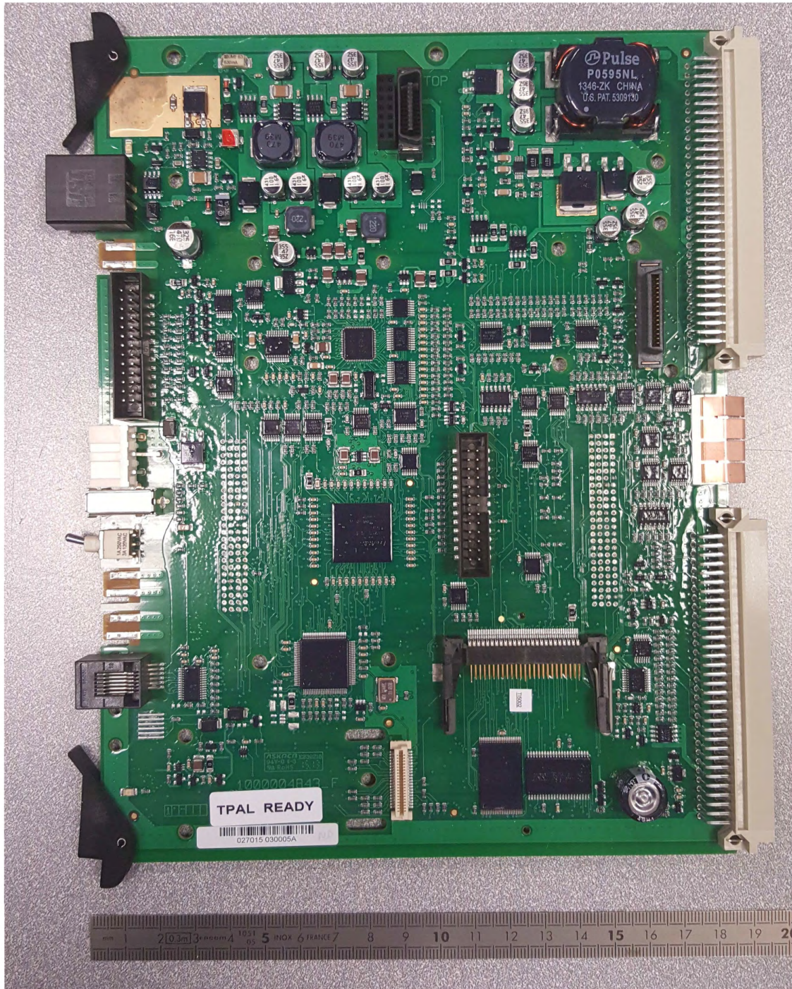
Main board Top
