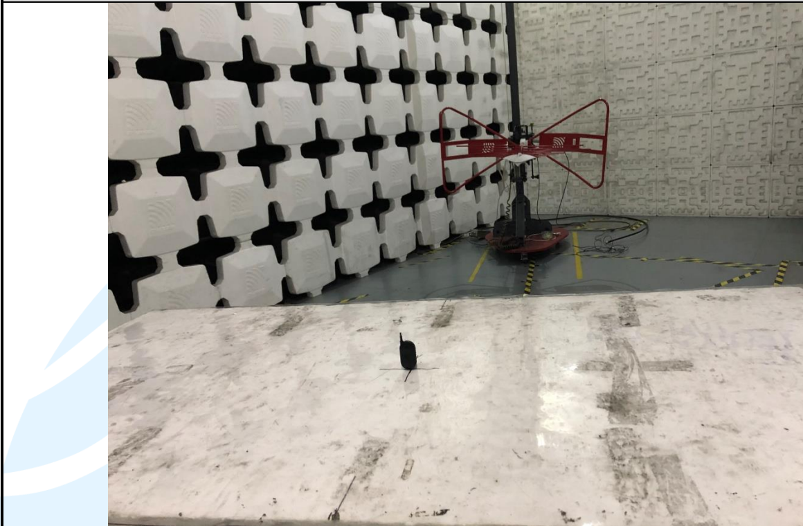
Radiated Spurious Emissions (30 MHz to 1000 MHz)
