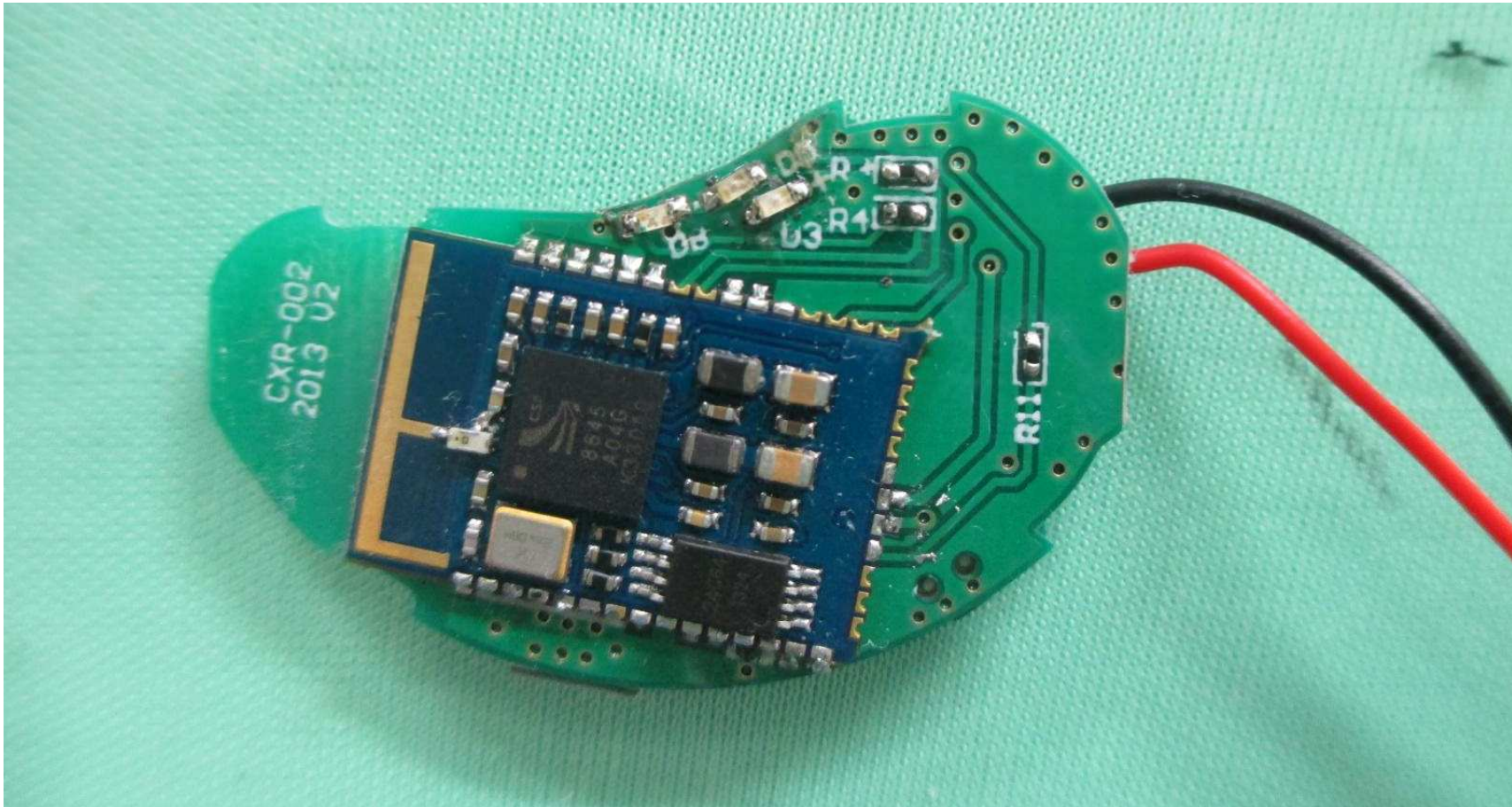
PHOTOGRAPH OF THE PRODUCT INNER CIRCUIT BOTTOM VIEW
