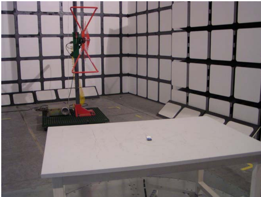
30 MHz – 1000 MHz: Radiated Emission - Front View
