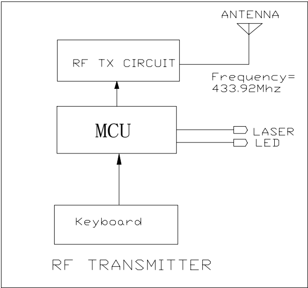
V9 Transmitter Block Diagram
