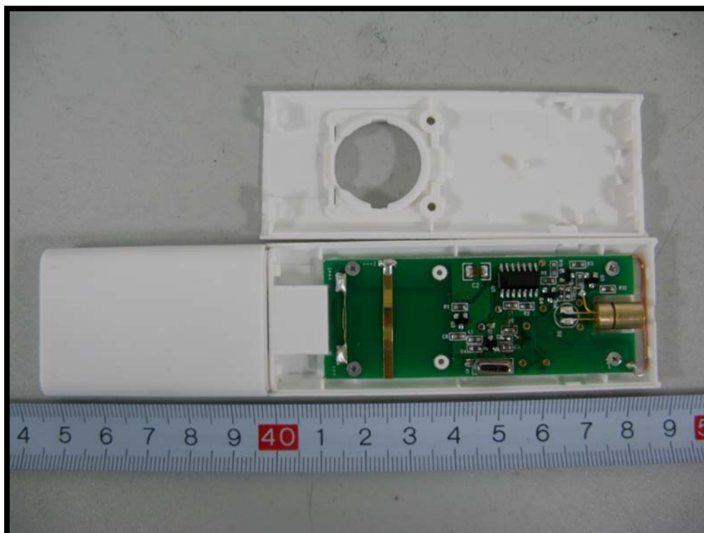
EUT-Uncovered View
