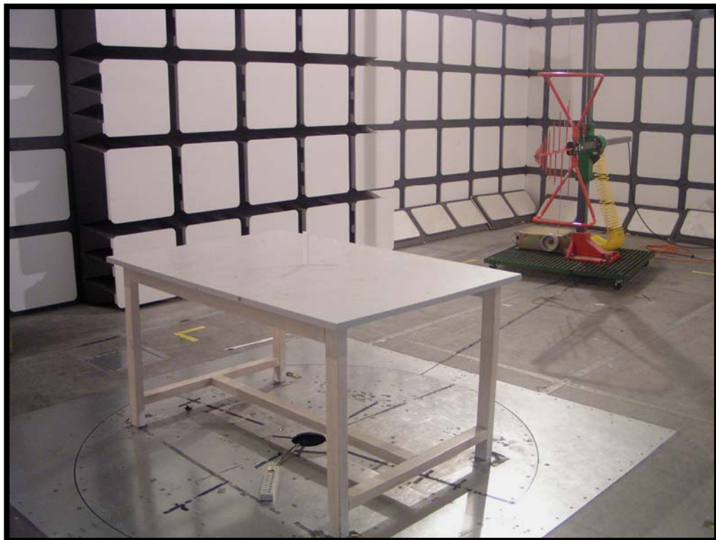
Radiated Emission - Rear View (Below 1 GHz)
