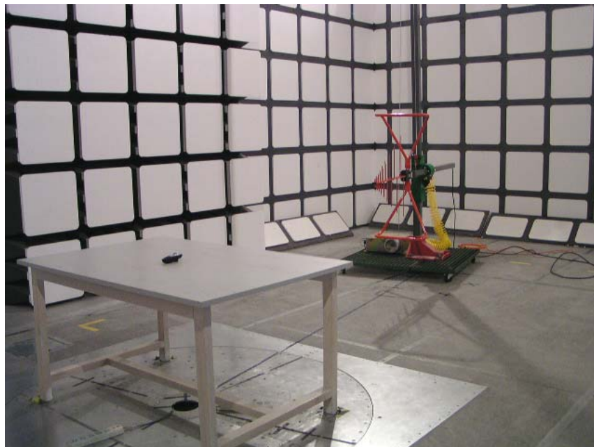
30 MHz – 1000 MHz: Radiated Emission - Rear View
