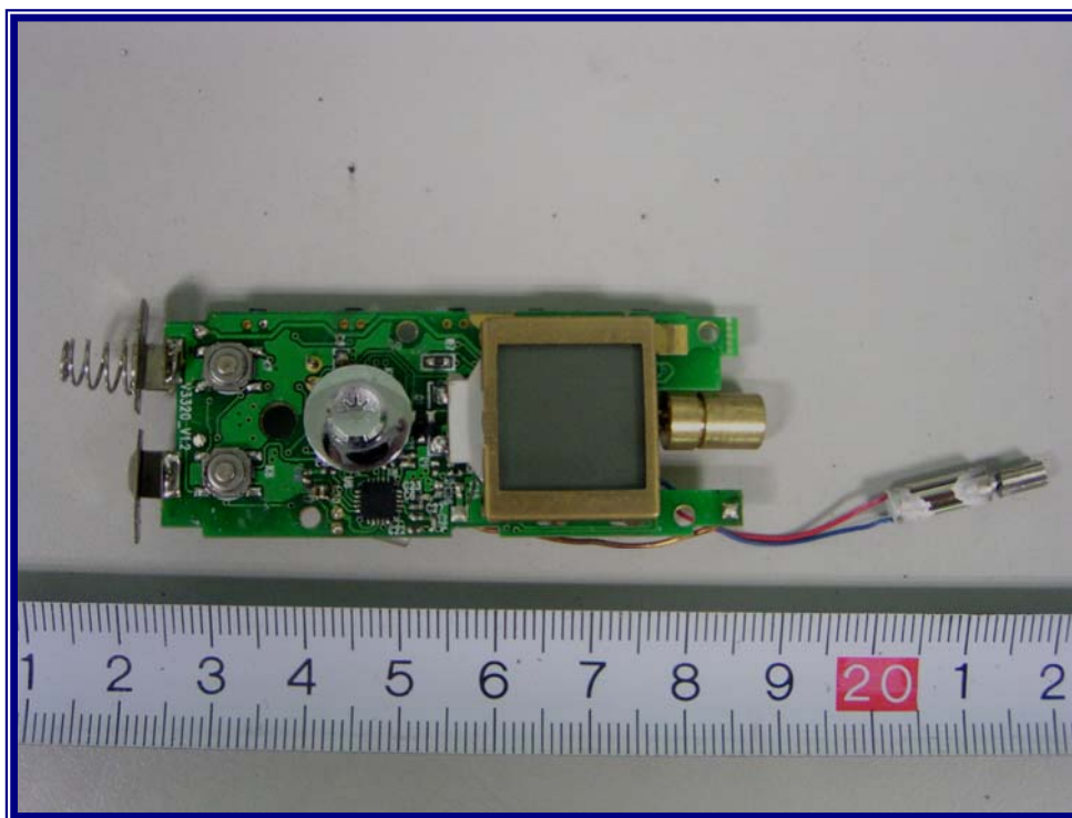
EUT- Main Component Board Top View
