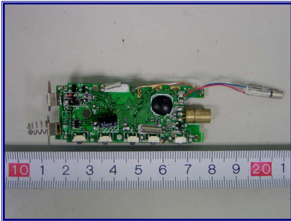
EUT- Main Component Board Bottom View
