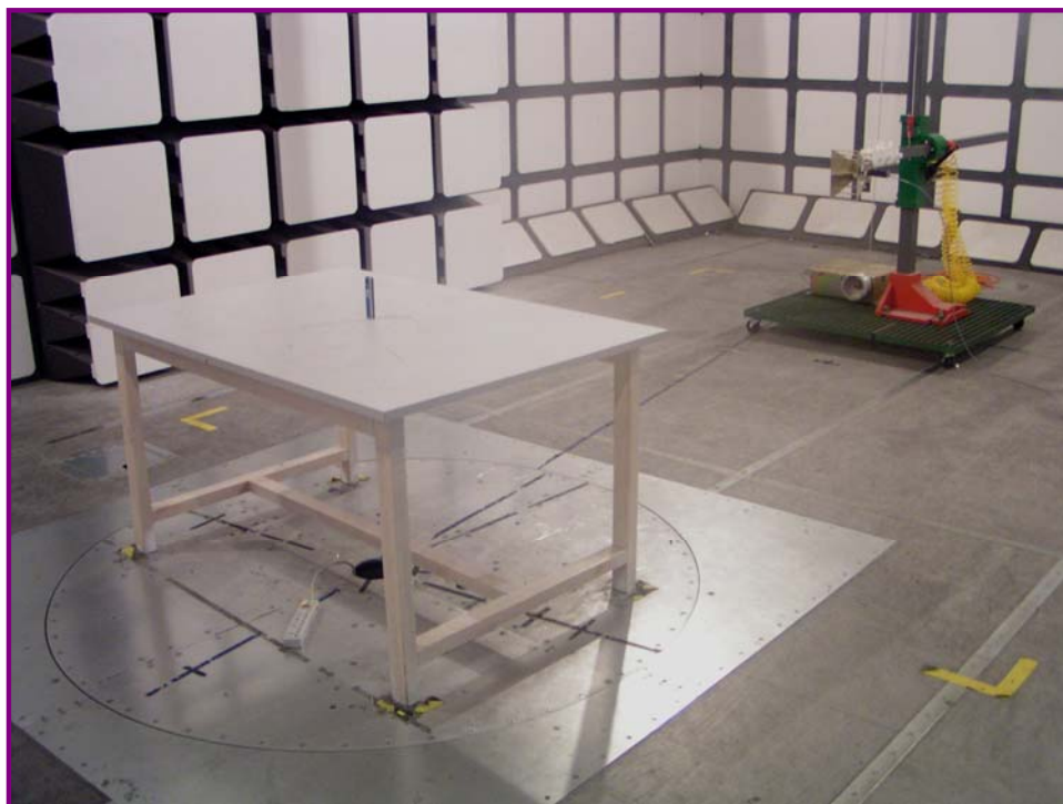
Radiated Emissions - Rear View (Above 1000 MHz)
