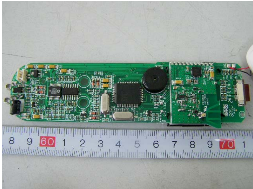
EUT- PCB Front View (Handset)
