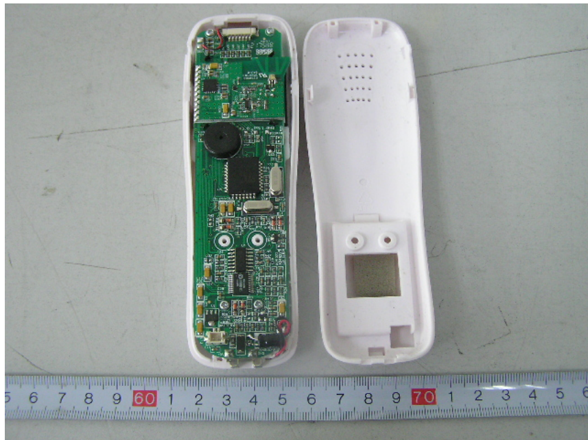
EUT- Cover off View (Handset)
