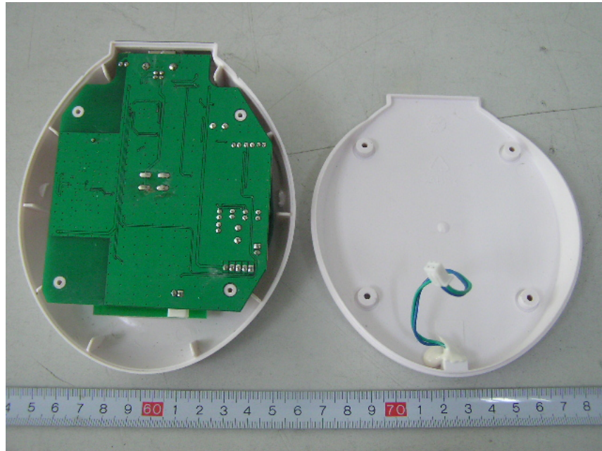
EUT- Cover off View (Base)
