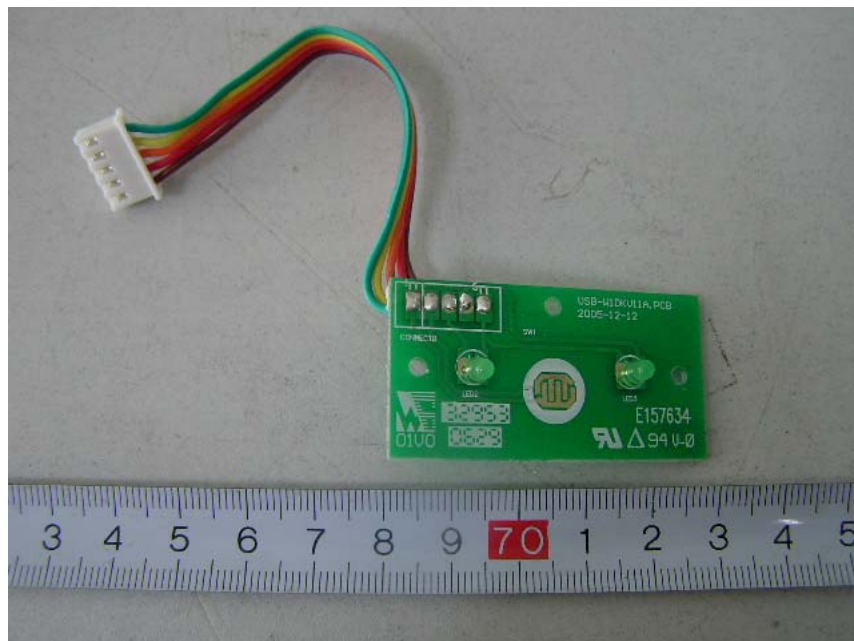
EUT- PCB 2 Front View (Base)
