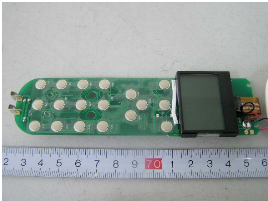
EUT- PCB Back View (Handset)
