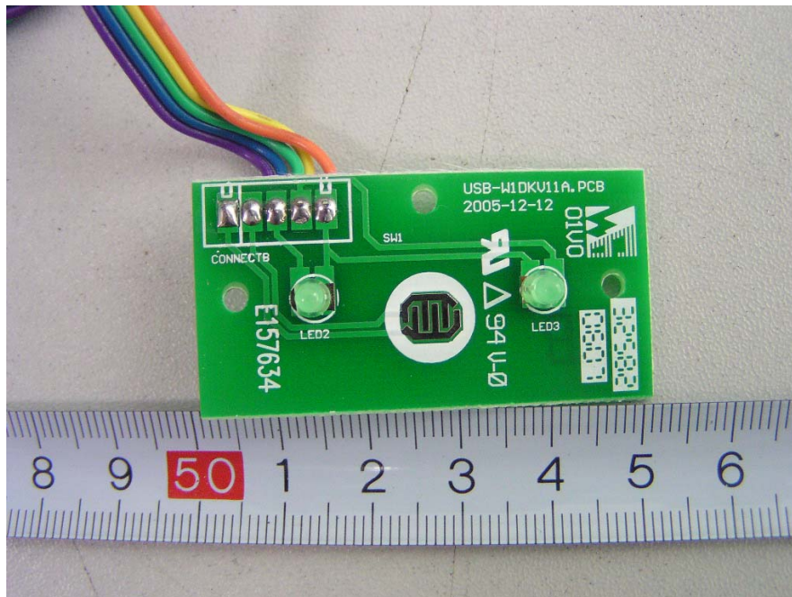
Handset – USB PCB Top View
