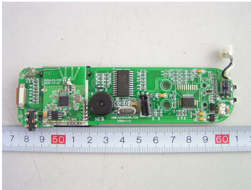
Handset –PCB Top View
