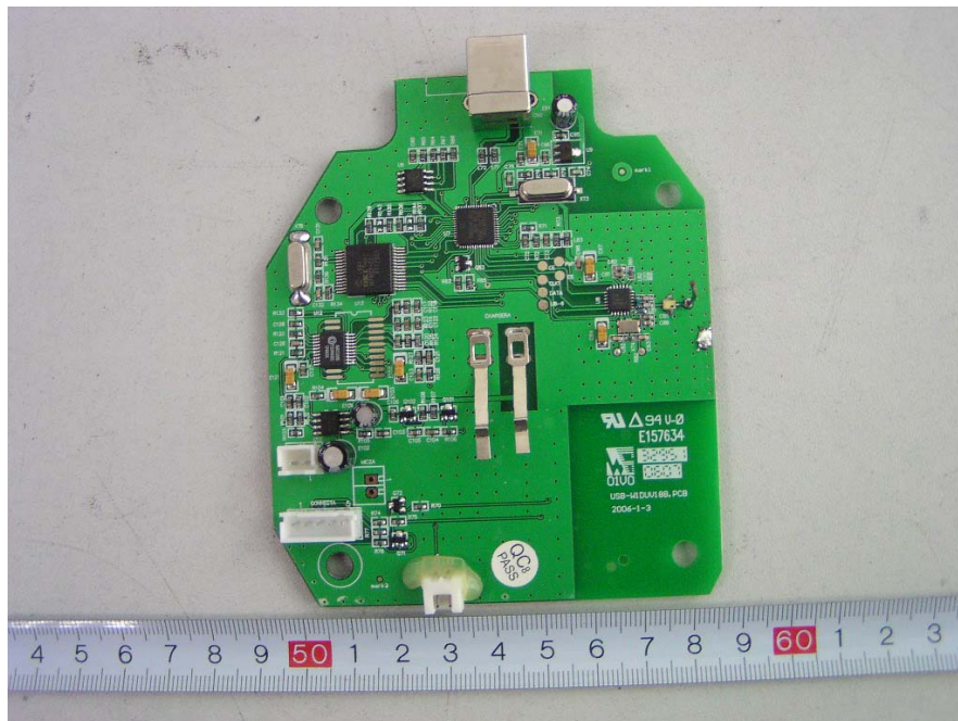
Base – Main PCB Top View
