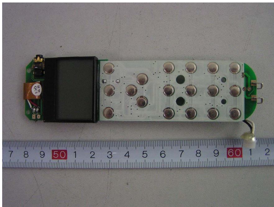
Handset –PCB Bottom View
