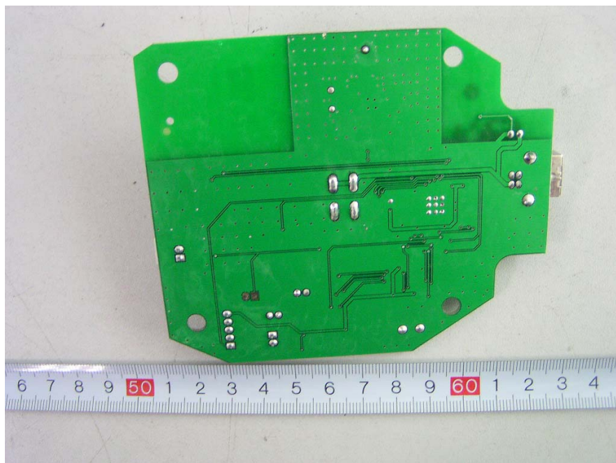
Base –Main PCB Bottom View
