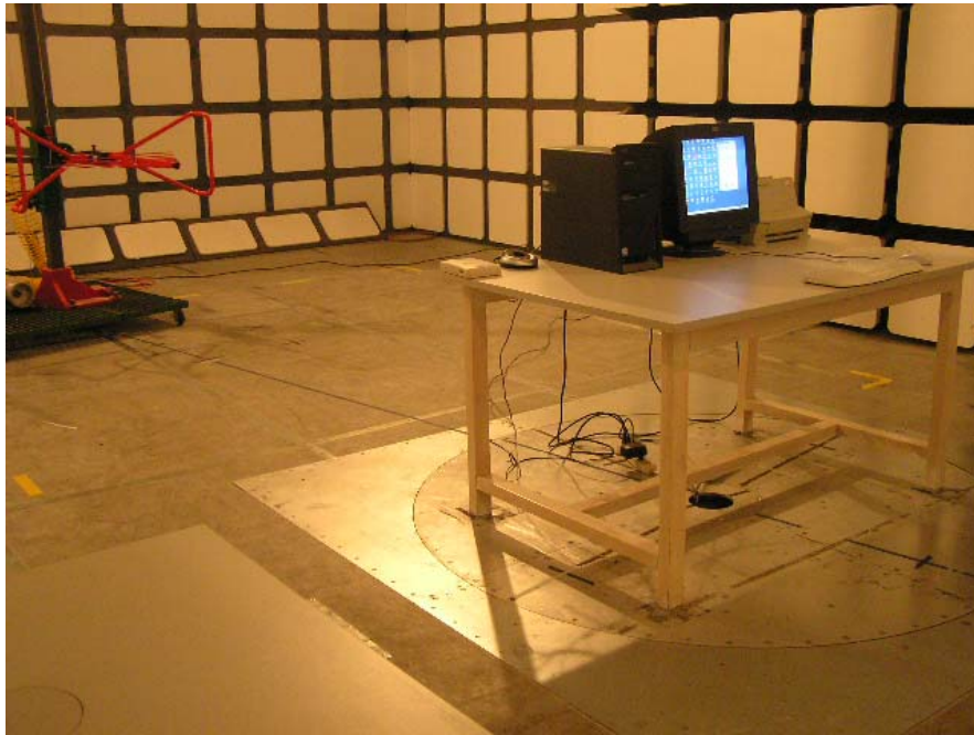
Base: Radiated Emission - Front View (30 MHz-1 GHz)
