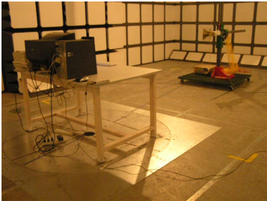
Base: Radiated Emission - Rear View (Above 1 GHz)
