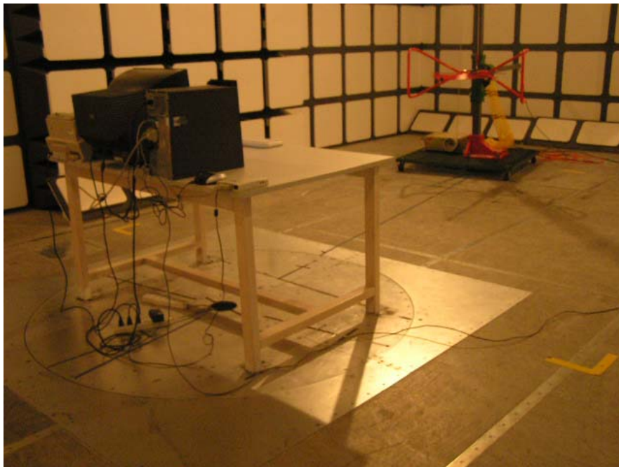
Base: Radiated Emission - Rear View (30 MHz-1 GHz)
