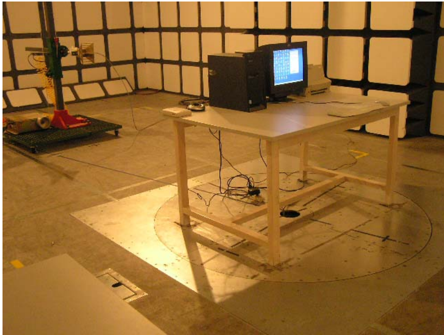
Base: Radiated Emission - Front View (Above 1 GHz)
