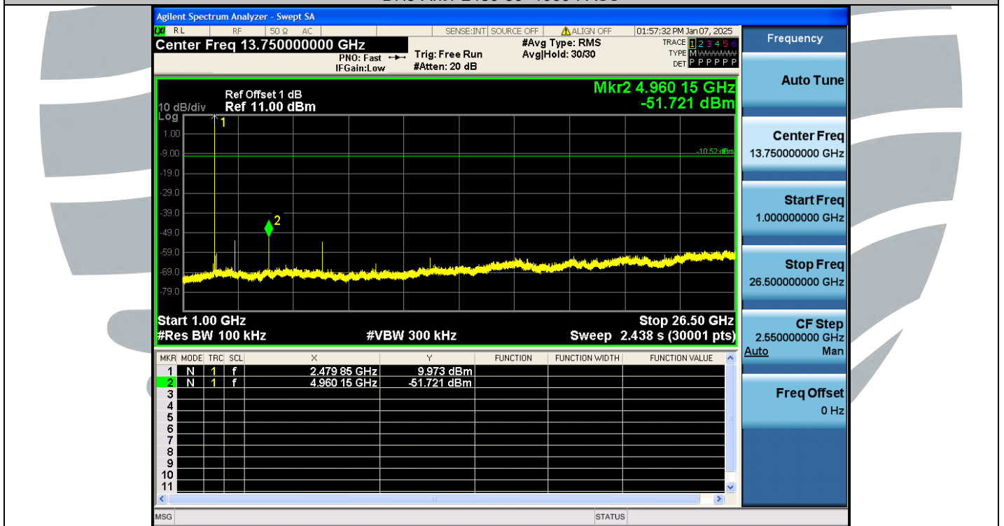
DH5-Ant1-2480-1000~26500-PASS
