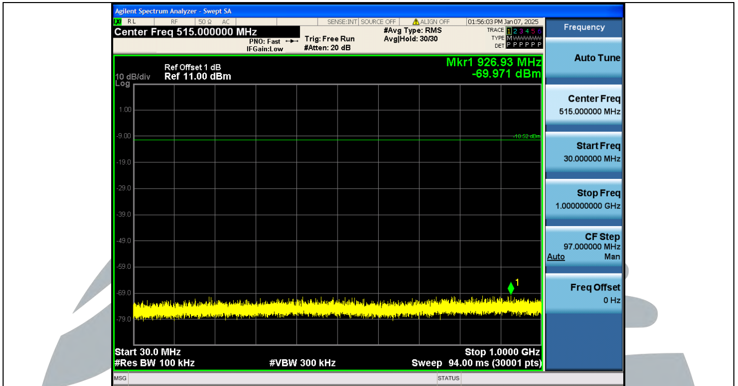
DH5-Ant1-2480-30~1000-PASS
