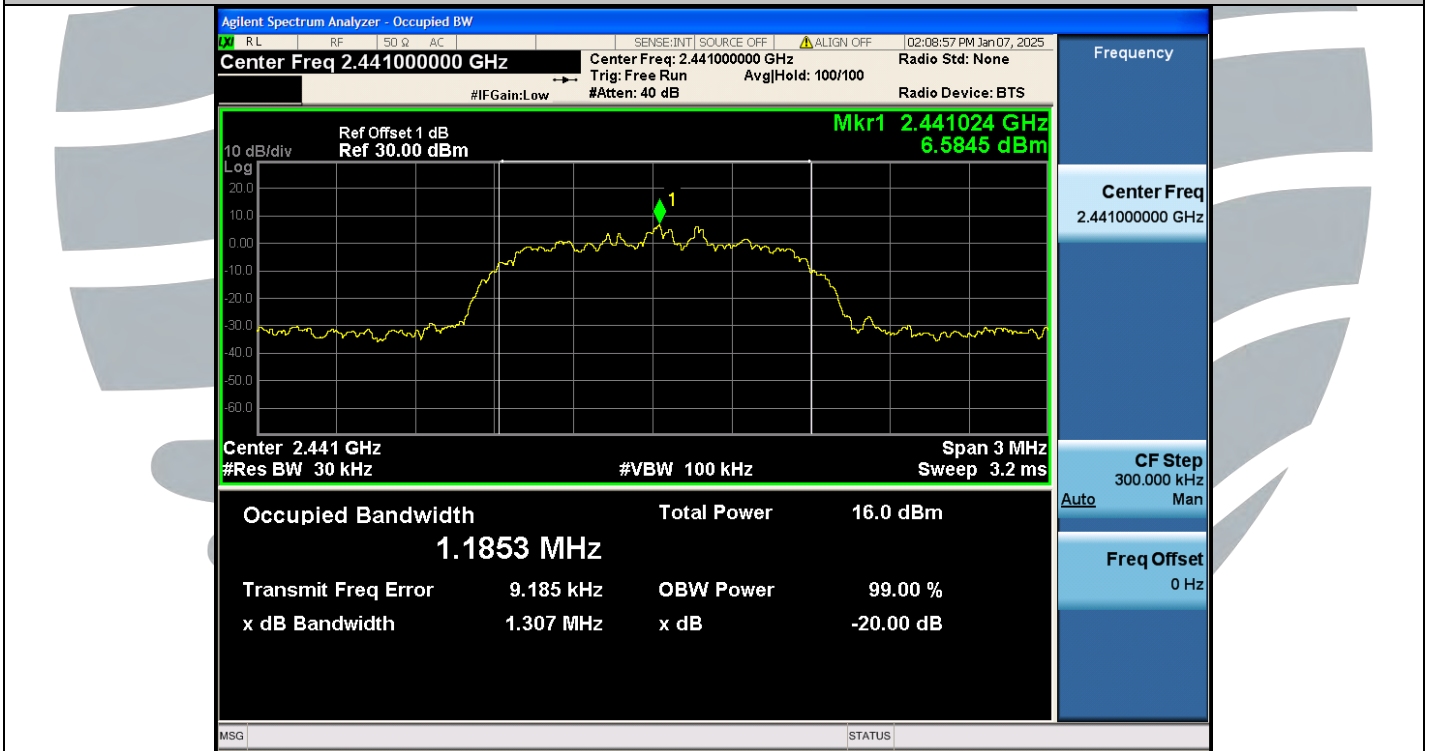
2DH5-Ant1-2441
