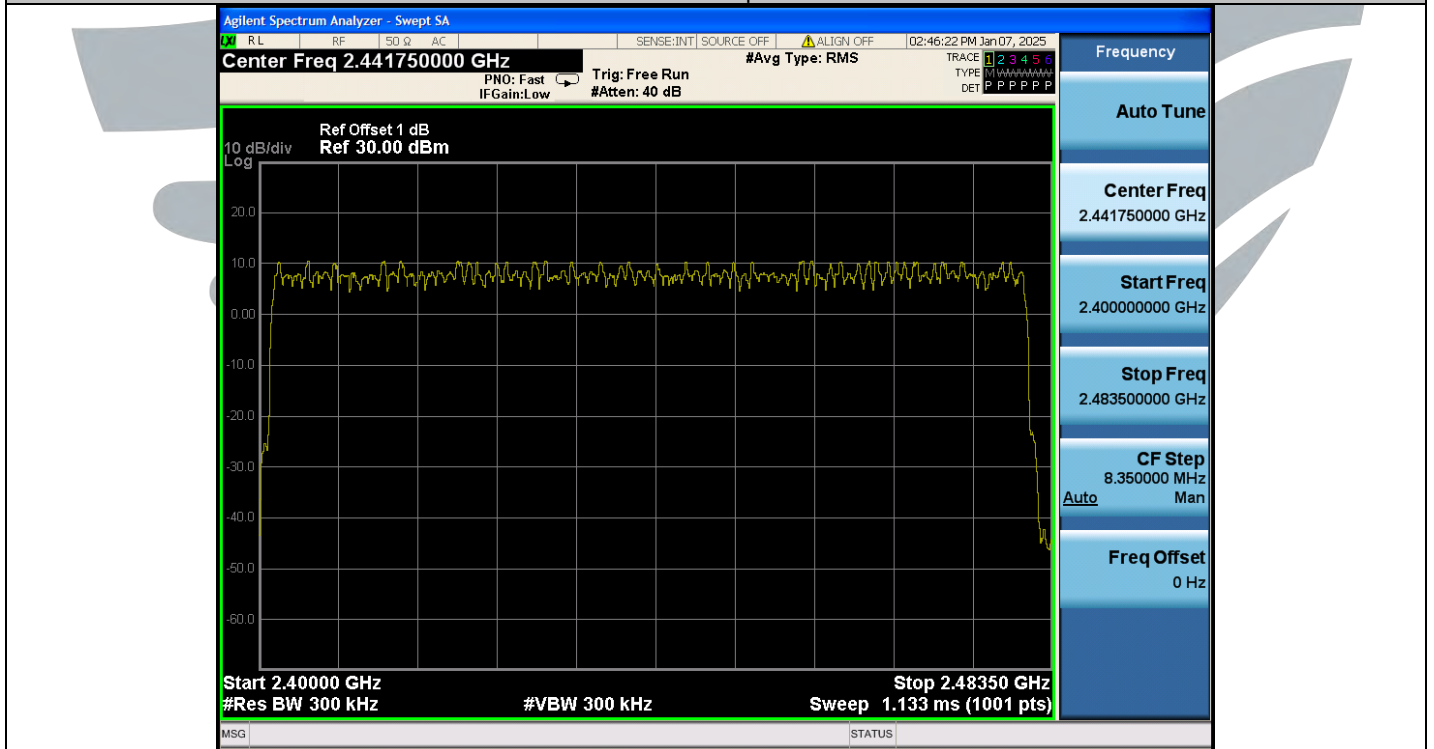
2DH5-Ant1-Hop-PASS
