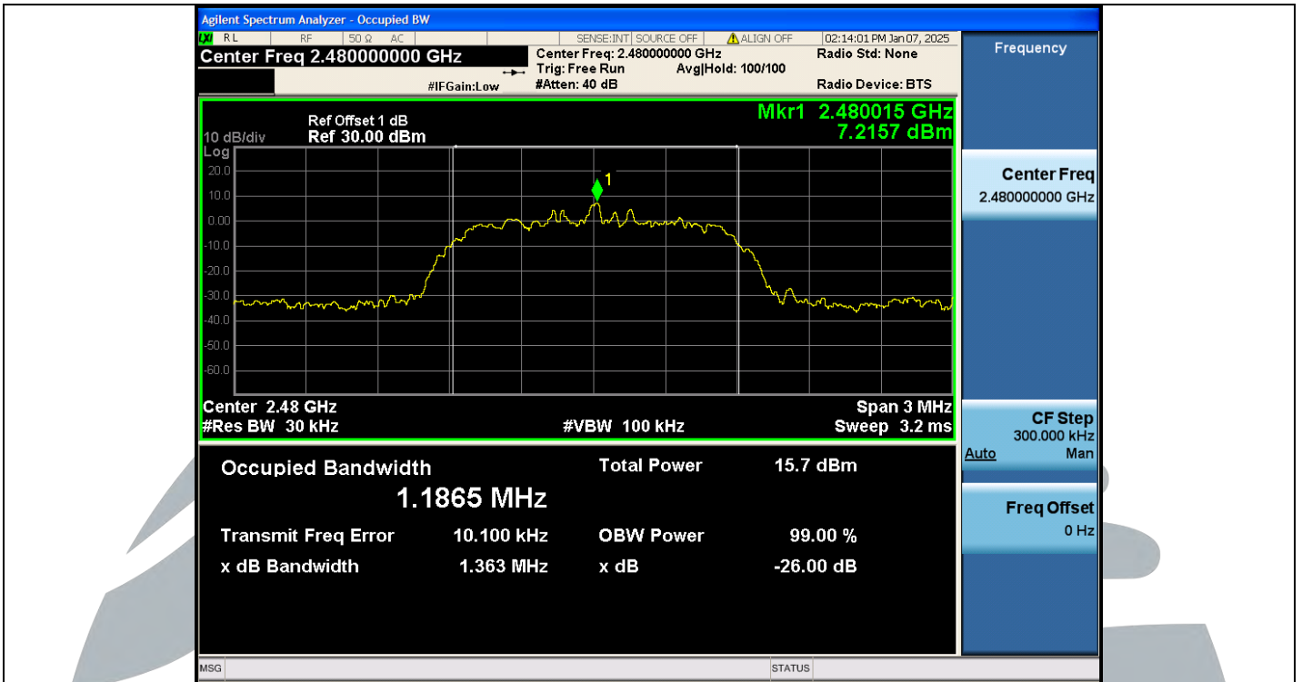
2DH5-Ant1-2480
