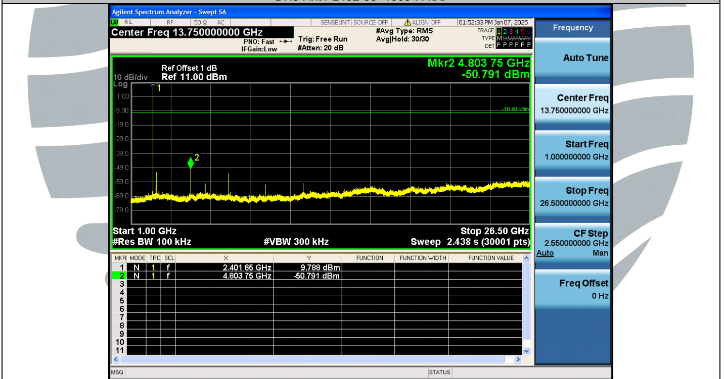
DH5-Ant1-2402-1000~26500-PASS
