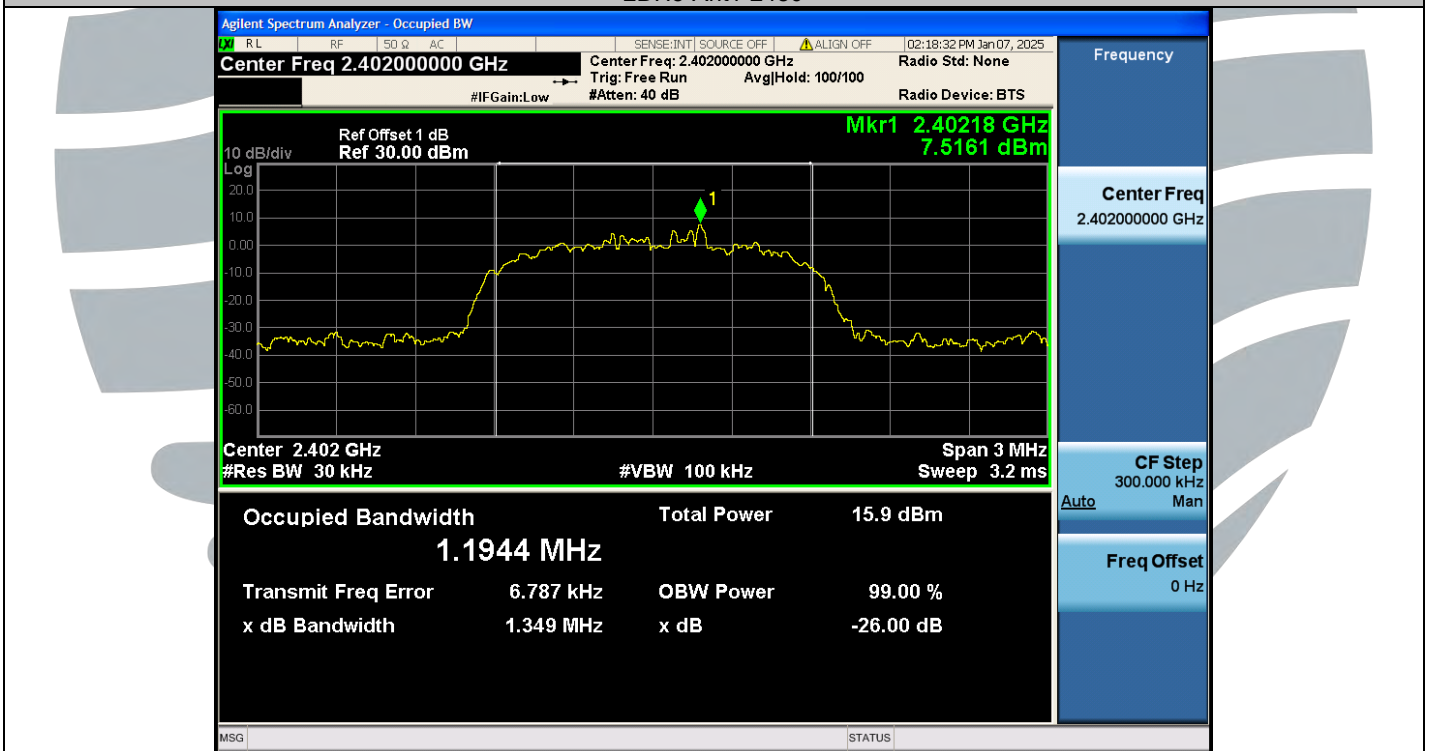
3DH5-Ant1-2402
