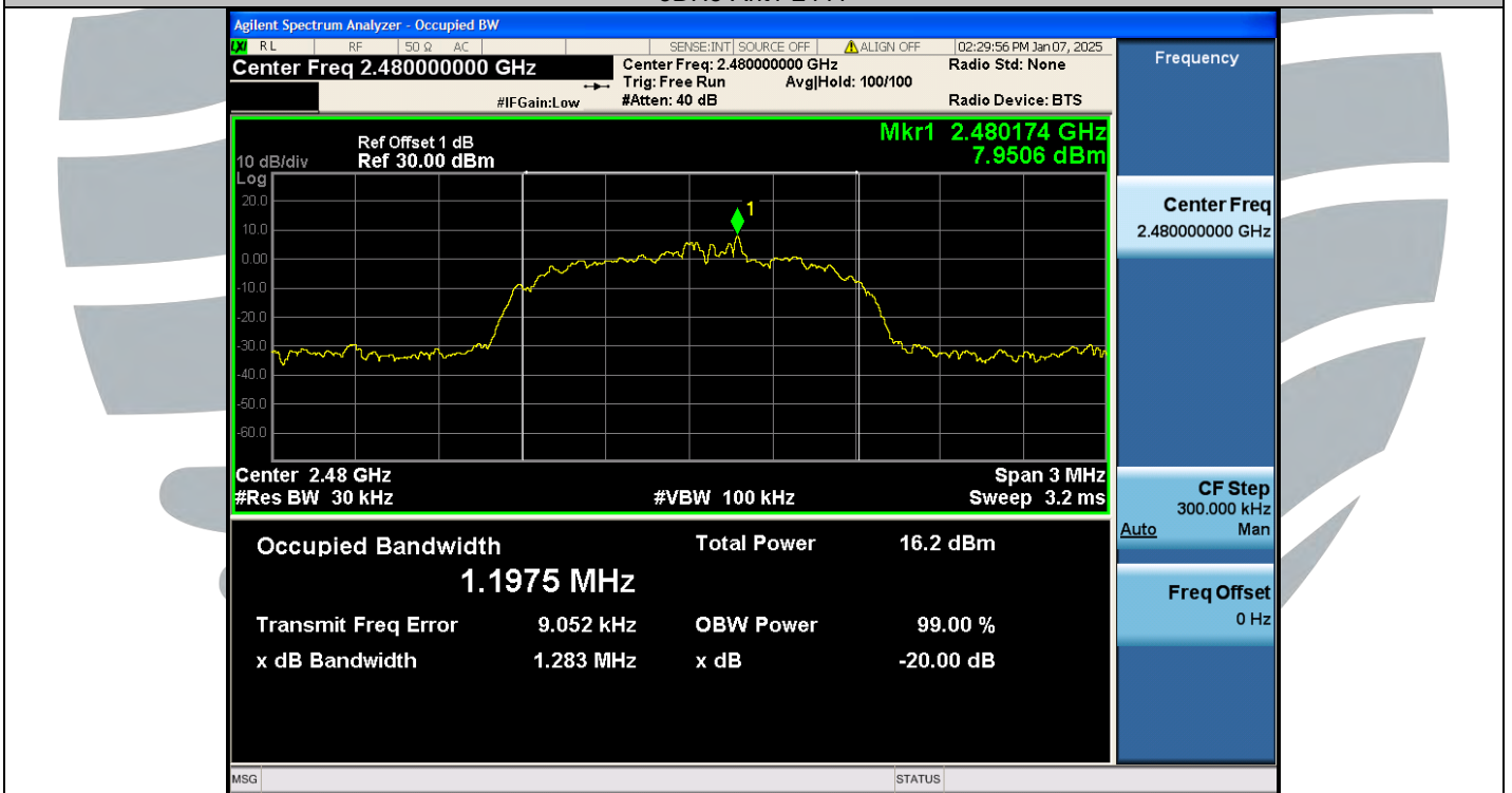
3DH5-Ant1-2480
