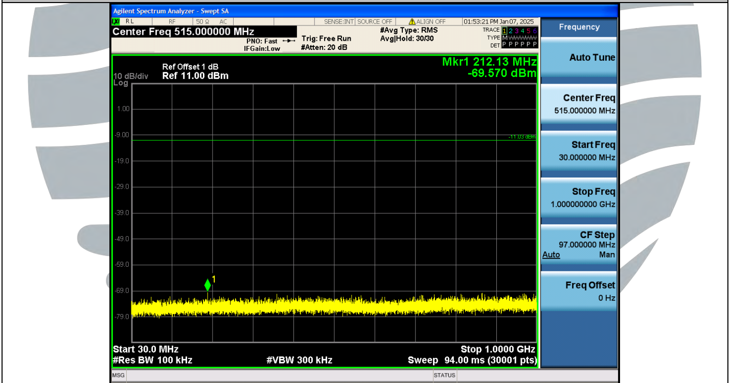
DH5-Ant1-2441-30~1000-PASS
