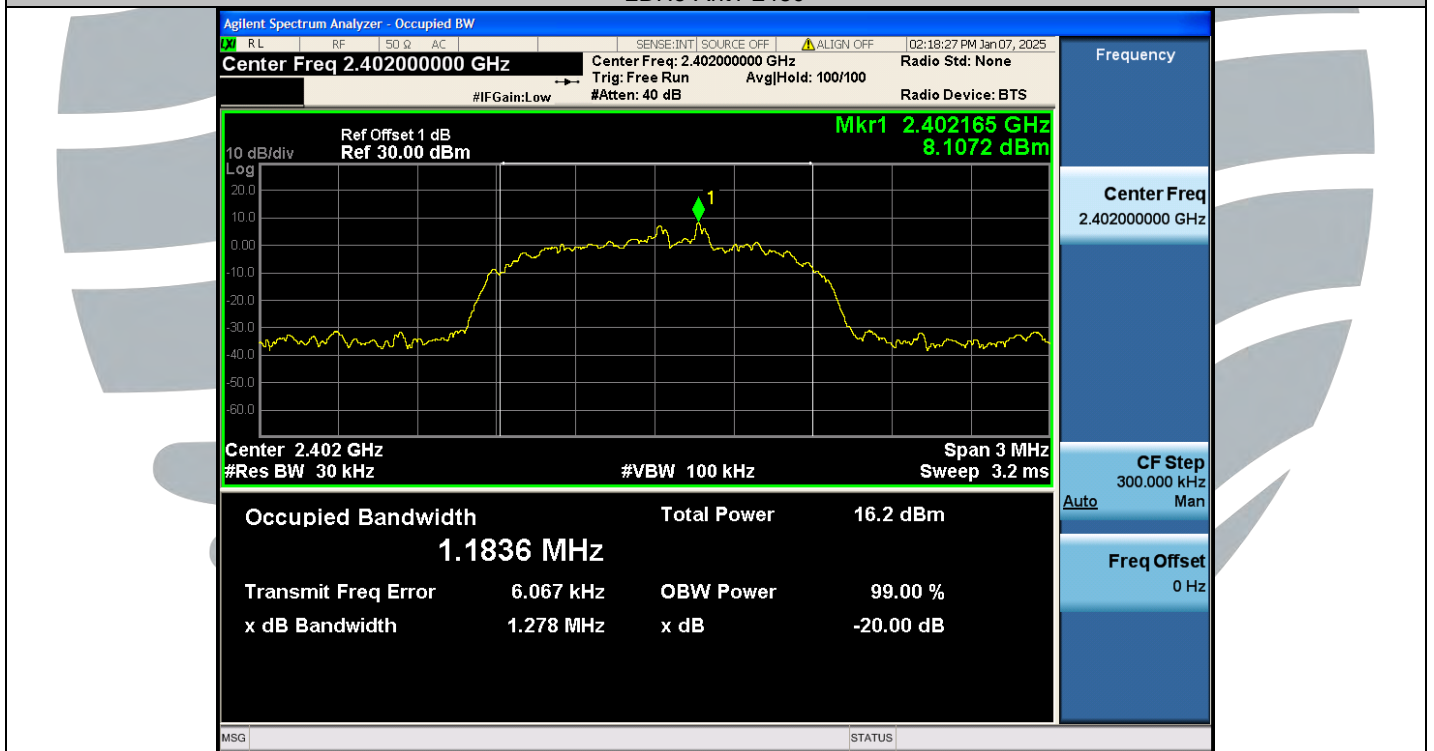
3DH5-Ant1-2402
