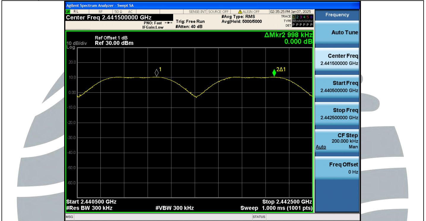
DH5-Ant1-Hop-PASS
