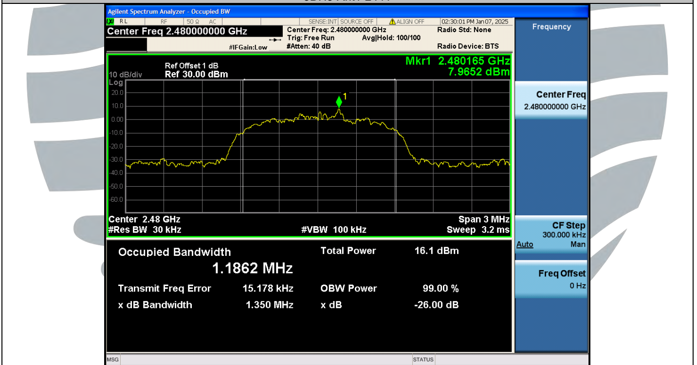
3DH5-Ant1-2480
