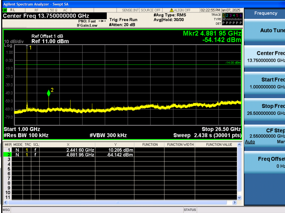
3DH5-Ant1-2441-1000~26500-PASS
