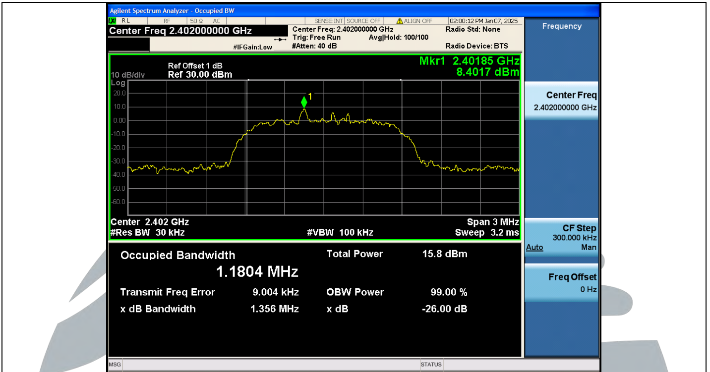
2DH5-Ant1-2402
