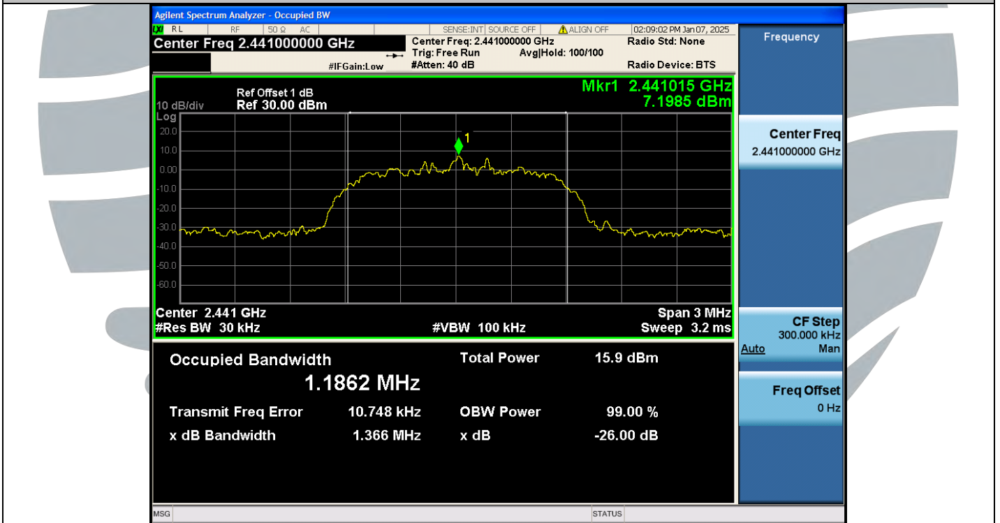
2DH5-Ant1-2441
