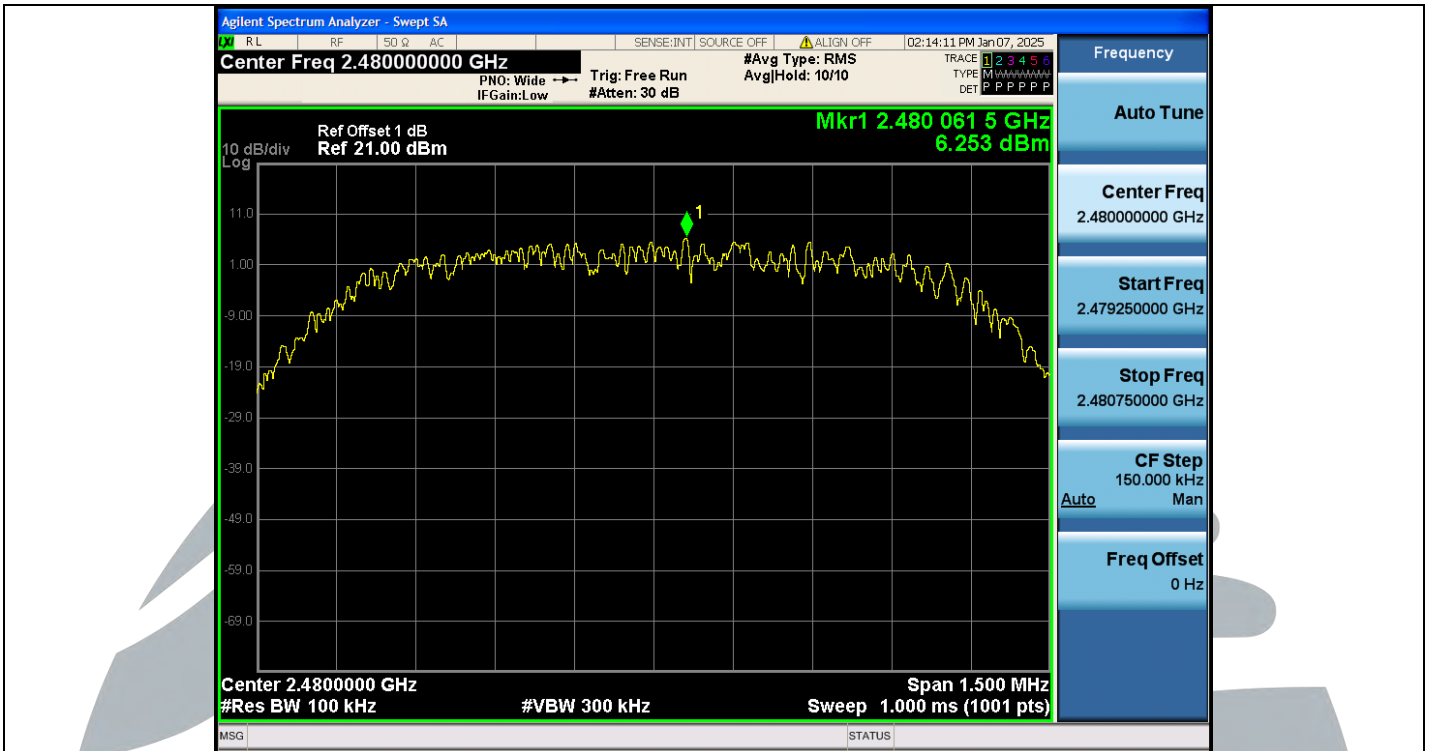
2DH5-Ant1-2480-0~Reference-PASS
