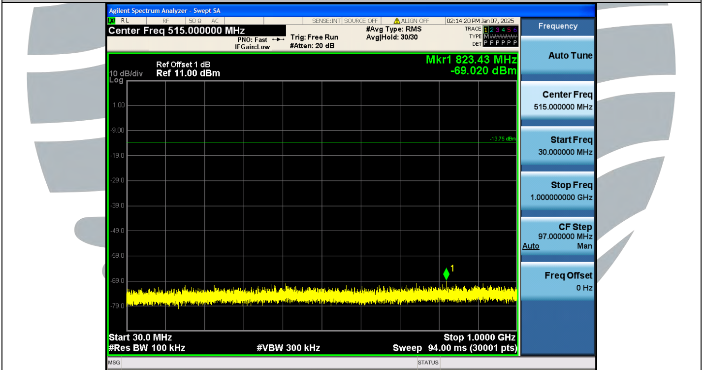
2DH5-Ant1-2480-30~1000-PASS
