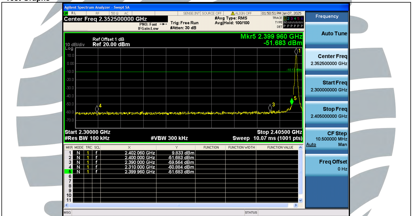
DH5-Ant1-2402-PASS
