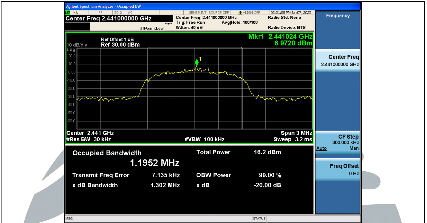
3DH5-Ant1-2441
