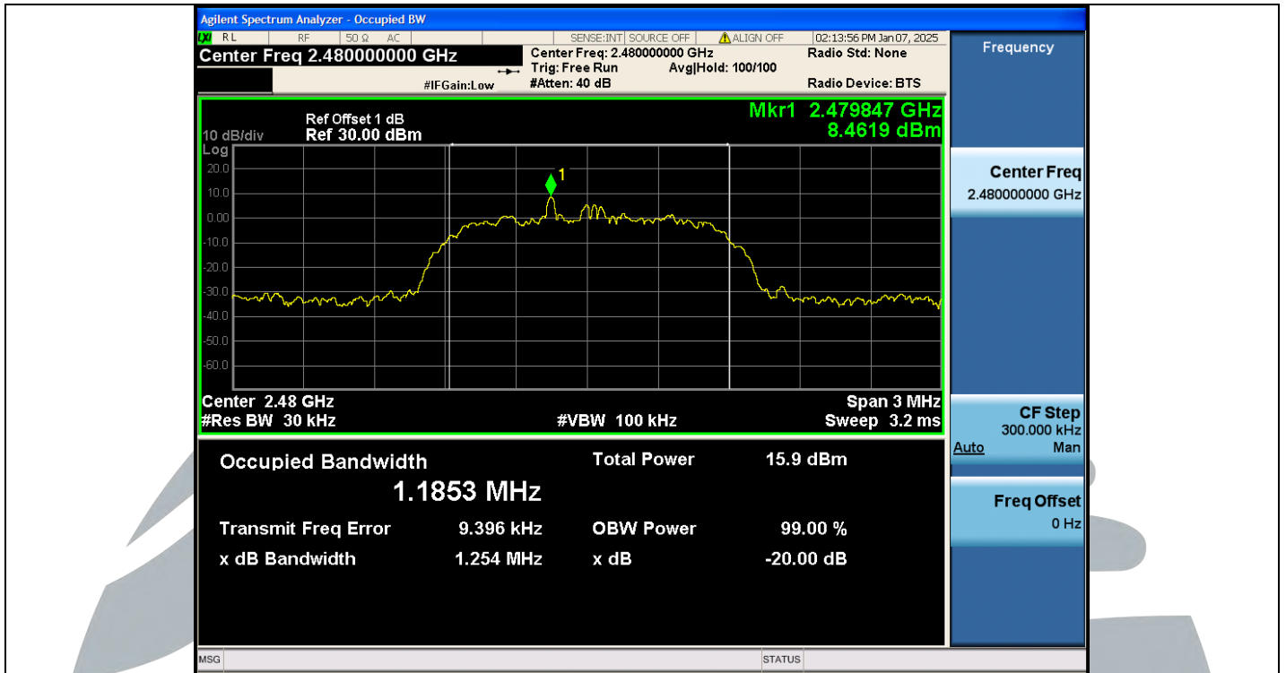
2DH5-Ant1-2480
