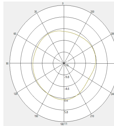
2D Antenna pattern (X->Y; X->Z; Y->Z)
