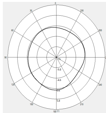
2D Antenna pattern (X->Y; X->Z; Y->Z)
