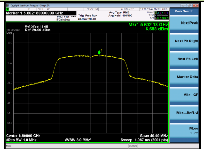
Channel 120 (5600MHz)
