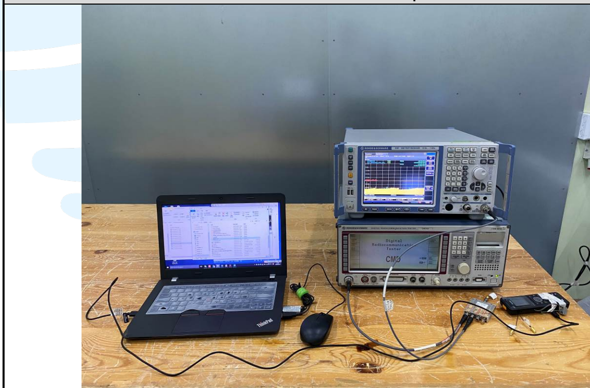
Conducted RF Test Setup
