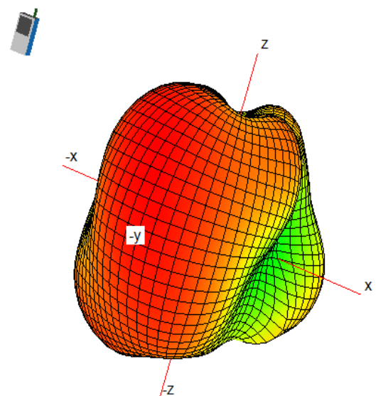
3D Antenna pattern
