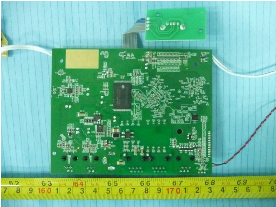
EUT – Main Board and USB Port Board Bottom View
