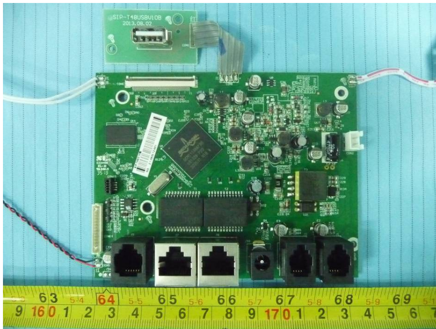
EUT – Main Board and USB Port Board Top View
