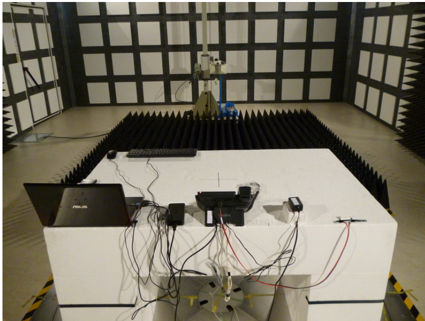
Radiated Emission - Rear View (Mode 2 above 1GHz)
