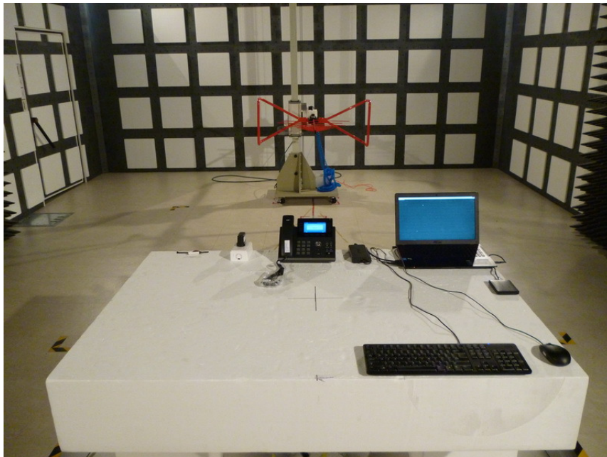
Radiated Emission - Front View (Mode 1 below 1GHz)
