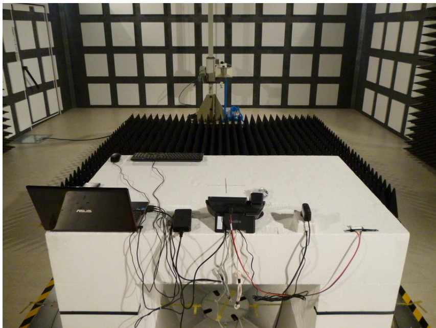
Radiated Emission - Rear View (Mode 1 above 1GHz)
