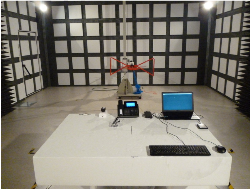
Radiated Emission - Front View (Mode 2 below 1GHz)
