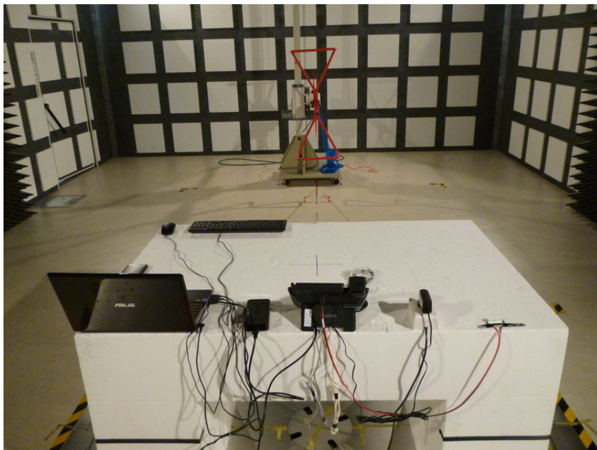
Radiated Emission - Rear View (Mode 1 below 1GHz)
