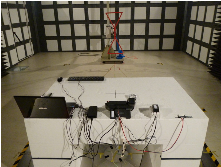
Radiated Emission - Rear View (Mode 2 below 1GHz)
