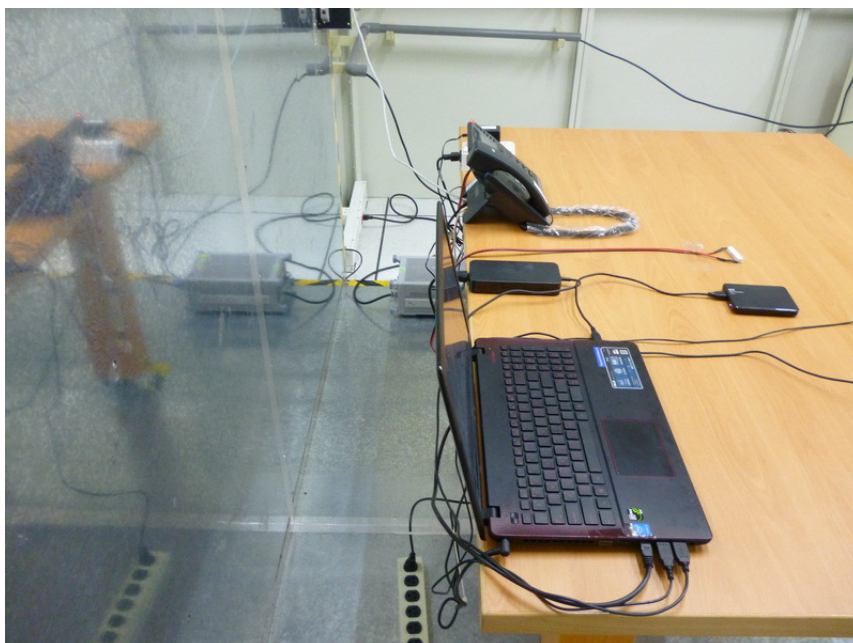
Conduction-Rear View (Mode 1)
