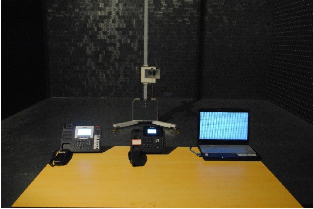
Radiated emission test view (1GHz Above)
