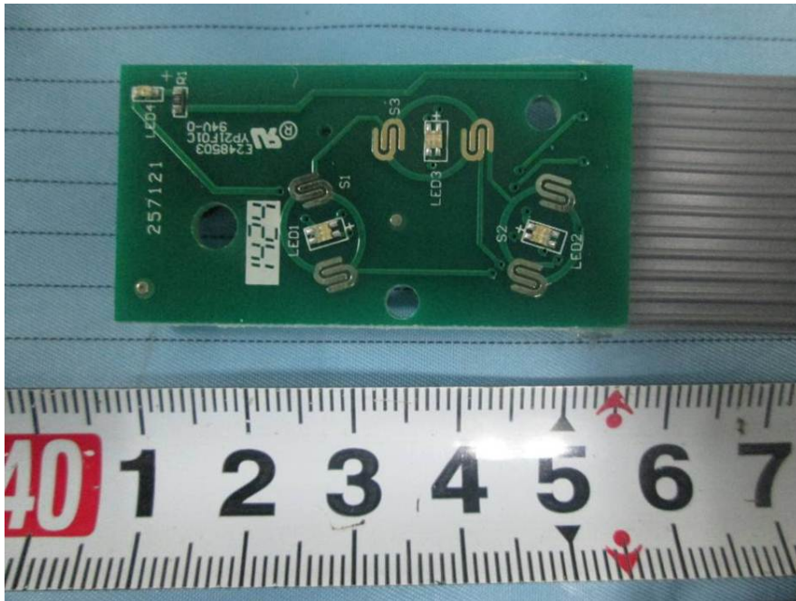
EUT – SIP-T23KB2V11A PCB Bottom View
