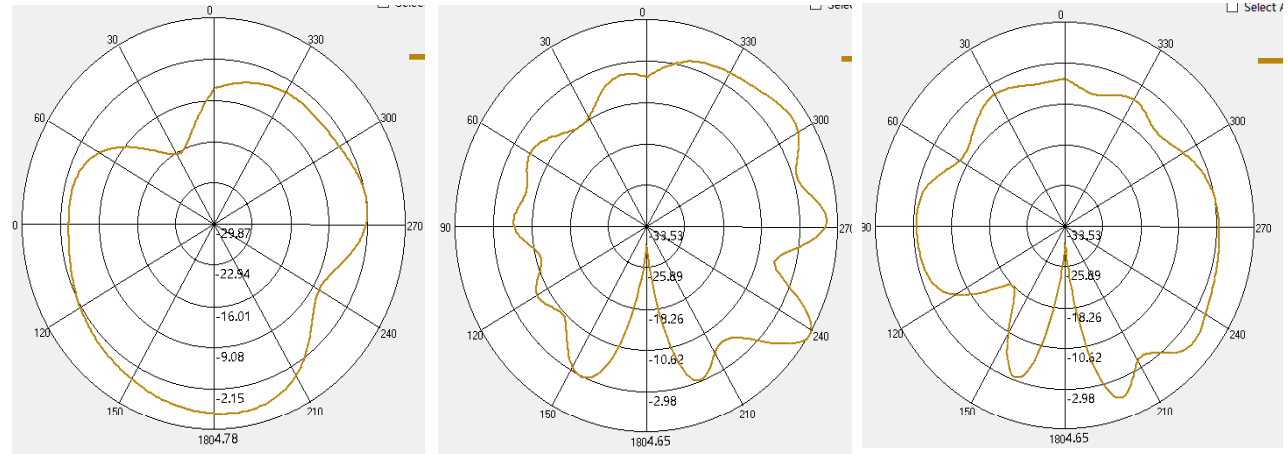
2D Antenna Pattern (X->Y; X->Z; Y->Z)
