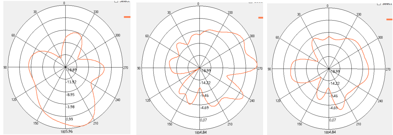
2D Antenna Pattern (X->Y;X->Z;Y->Z)
