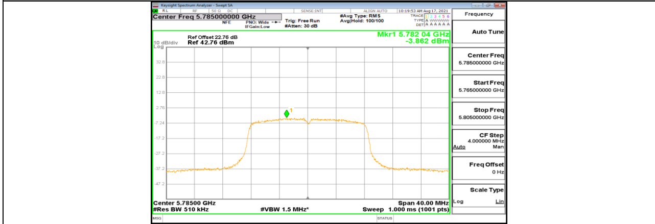
11A-CDD_Ant2_5785
