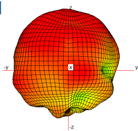
3D Antenna Pattern
