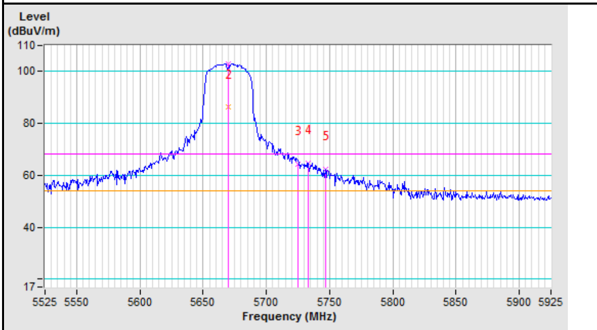
5670MHz Vertical
