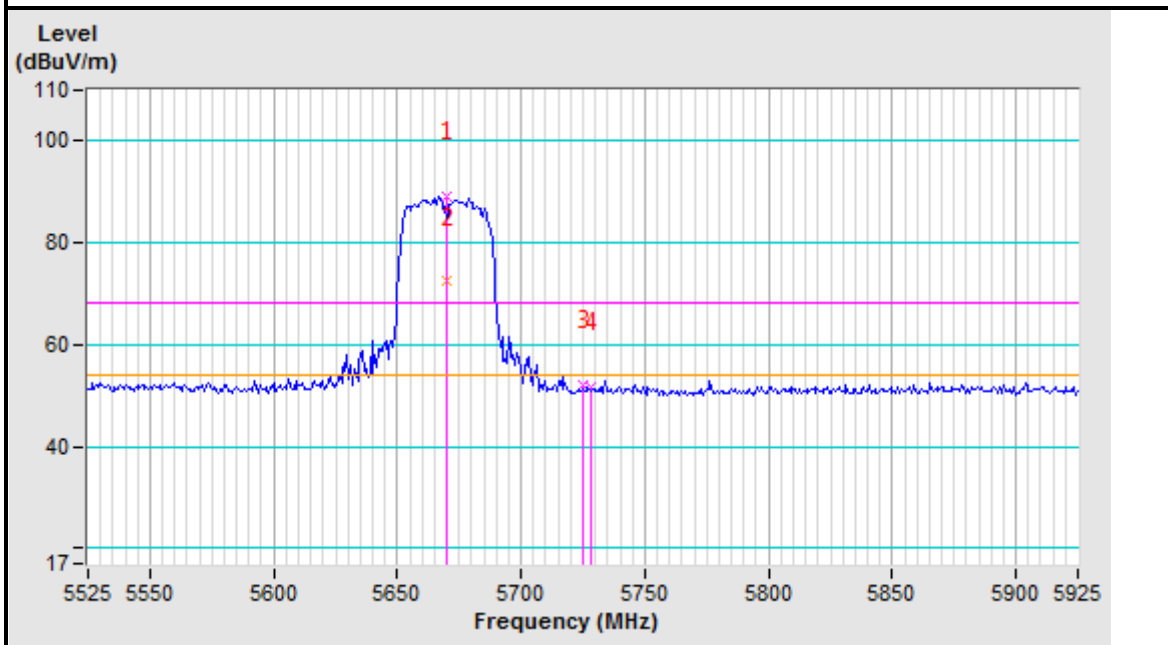
5670MHz Vertical
