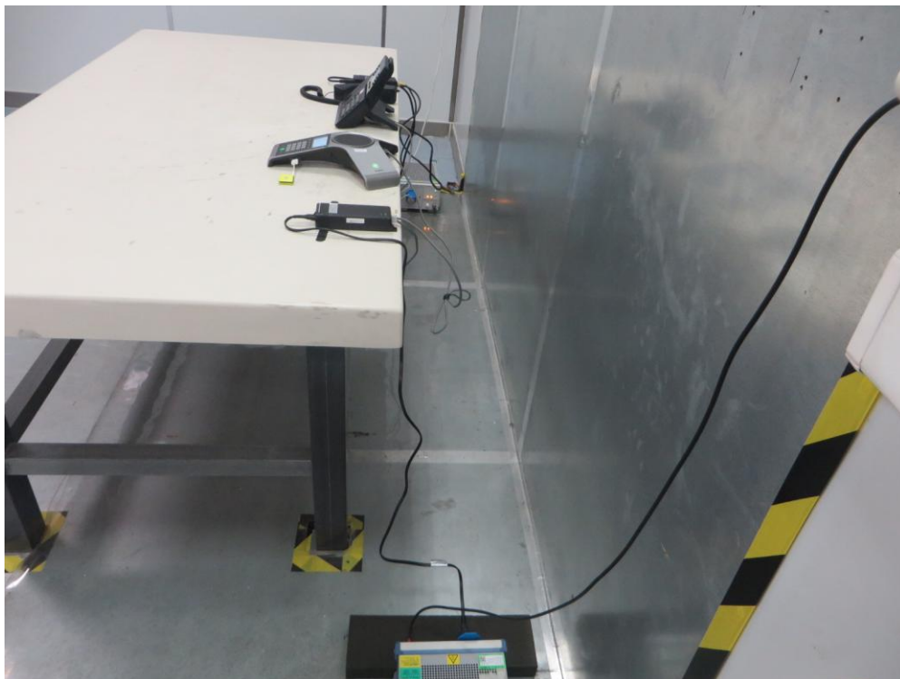
Description: Back View of Conducted Emission Test Setup for Mode 2
